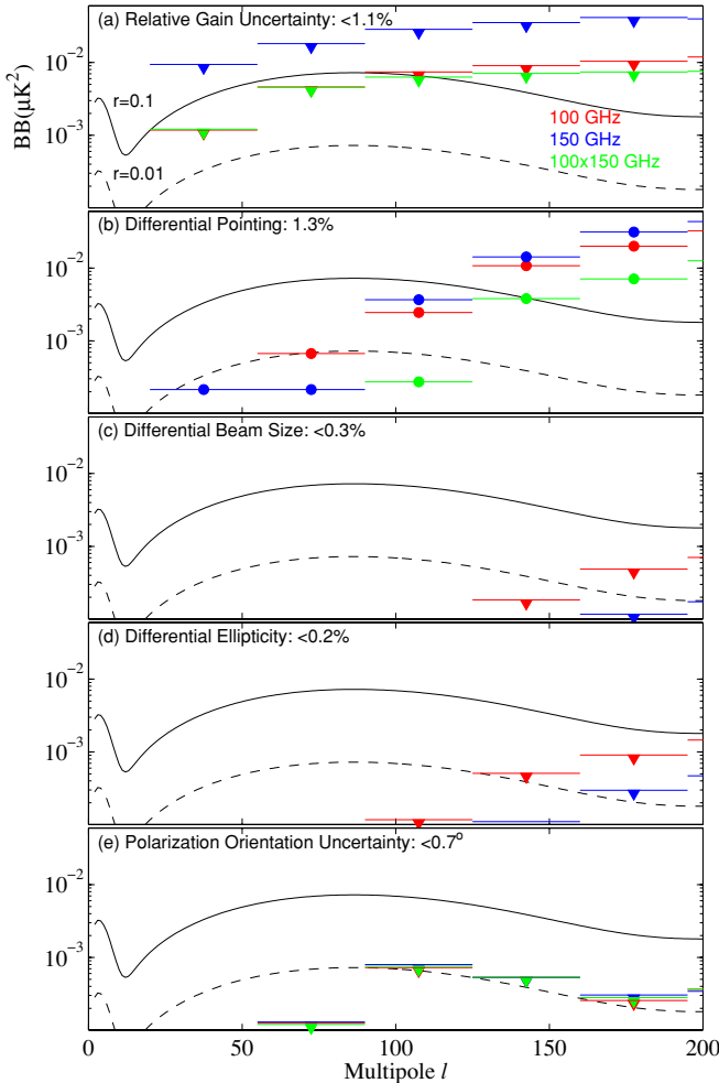
Figure 10. Spurious BB power from simulations of measured potential systematic errors. Except for differential pointing, all BB estimates correspond to measured upper limits. Effects of relative gain error and differential pointing can be corrected for in the analysis if necessary. All the potential systematic uncertainties are measured to be well below the two-year constraint of r < 0.72 (Chiang et al. 2010).
