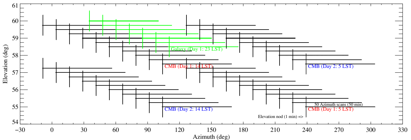
Figure 3. 48 hr observing cycle consists of 6 hr for cycling the refrigerator (not shown), two 9 hr blocks of raster scans on our main CMB field on the first day, a 6 hr block of similar raster scans on the Galaxy, and two more 9 hr blocks on the main CMB field on the second day. Each of the upper and lower halves of the elevation range is scanned in different azimuth ranges between the two days, allowing a jackknife test for ground contamination. At the beginning and end of each set of 50 minute azimuth scans, a \pm 0.6 elevation “nod” is performed to measure relative gains of every bolometer. This 48 hr cycle is repeated at different boresight rotation angles: \{-45^\circ, 0^\circ, 135^\circ, 180^\circ\} .
