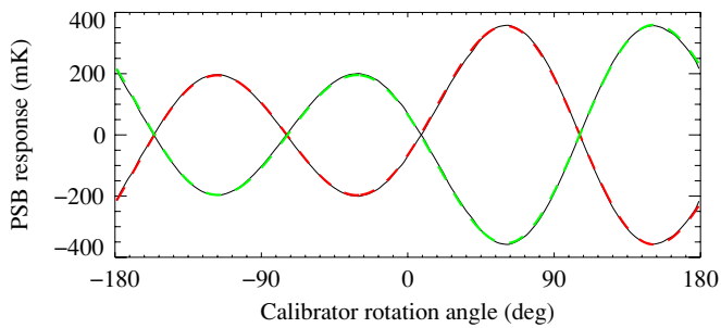
Figure 12. Response of each PSB in a pair as a function of the dielectric sheet calibrator orientation (black), plotted over by the fits (in red/green dashes) with polarization orientations and responsivities as free parameters.
