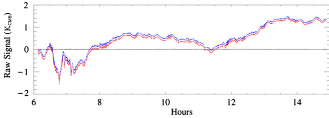
Figure 6. Individual 150 GHz timestreams within a PSB pair (red and blue) are differenced (black) in this plot using a single relative gain fit over the plotted 9 hr period. For the actual CMB analysis, relative gains are updated for every 1 hr scan set.
