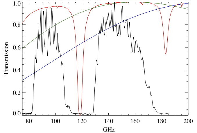
Figure 7. Average measured spectral response for each of BICEP’s frequency bands, normalized to unity. Overplotted are the atmospheric transmission at the South Pole (red), the CMB spectrum (green), and its temperature derivative (blue).
