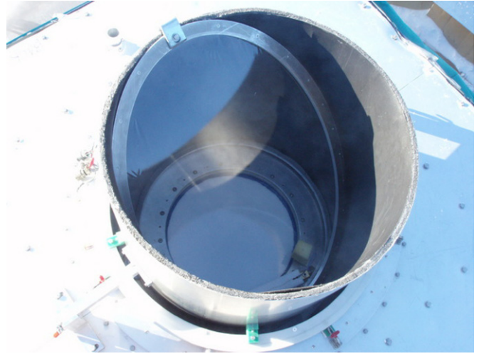
Figure 11. Dielectric sheet calibrator for measuring PSB orientations consists of a beam-filling polypropylene sheet and an ambient load made of a highly emissive black lining, subjecting the beams to partially polarized radiation. The device is mounted on the azimuth stage, which can rotate about the telescope's boresight when pointed at zenith.
