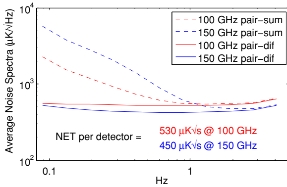
Figure 19. Average noise power spectra of all PSB pairs used in the analysis, averaged over all observing blocks during the entire first two years. The pair-sum spectra show 1/f atmospheric noise, which is rejected by pair differencing. NETs per detector are derived from the pair-difference average between 0.1 and 1 Hz. Accounting for polarization efficiencies, these correspond to an average instantaneous (i.e., single Stokes parameter) “NEQ per feed” of 410 and 340 \mu\text{K}\sqrt{\text{s}} for 100 and 150 GHz, respectively.
