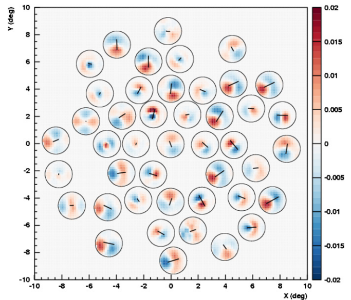
Figure 9. Beams for each PSB pair are normalized and differenced to produce this composite differential beam map (in the same orientation as Figure 2). The overlotted lines show the fitted pointing offsets magnified by a factor of 100.
