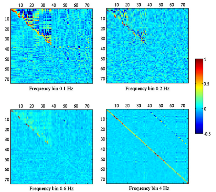
Figure 20. Example correlation matrices from the BICEP noise model. Each panel shows the fractional cross-correlations among PSB sums (indexes 1–37) and differences (indexes 38–74) of 37 PSB pairs used in 2007, with the real and imaginary components plotted in the upper right and lower left halves, respectively. The auto-spectra values along the diagonal are normalized simply by the maximum of the 74 values. The atmosphere-induced correlations are visible as off-diagonal structure among the pair sums. The imaginary component lacks substantial power, except among the pair sums at the lowest frequencies where the correlations due to atmosphere can be phase shifted depending on the relative beam locations. We define the noise model in 12 frequency bands spanning 0.05–5 Hz, and four of those bands are shown.
