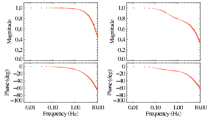
Figure 5. Measured transfer functions for a representative PSB (left) and an anomalous PSB (right), with error bars showing rms measurement repeatability. Most of the anomalous transfer functions are well described by Equation (2) and are repeatably measured, but are conservatively excluded from the initial analysis.
