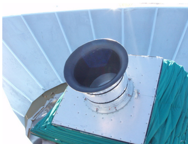
Figure 15. Absorptive forebaffle and the reflective ground screen.
