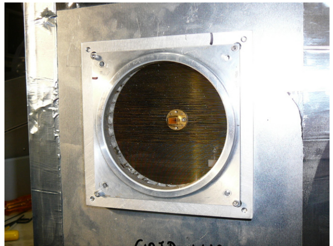
Figure 14. Another calibration source, used on top of a mast, for measuring cross-polarization responses (and PSB orientations). The broadband noise source at 100 or 150 \text{ GHz} outputs power through the rectangular feedhorn oriented for either vertical or horizontal polarization and through a precisely aligned wire grid to minimize cross-polarized signal.
