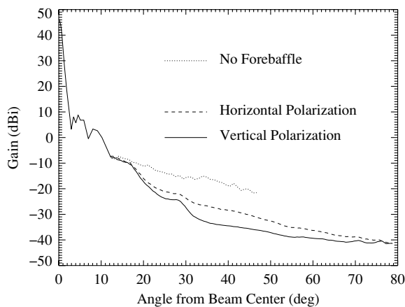
Figure 17. Azimuthally averaged sidelobe response for the 100 GHz central feed. A forebaffle with an absorptive lining cuts in at 15.5^\circ and provides up to an additional \sim 15 dB attenuation. When the telescope is at its lowest elevation of 50^\circ , the lip of the outer ground screen is \sim 30^\circ from the beam center of the central feed.
