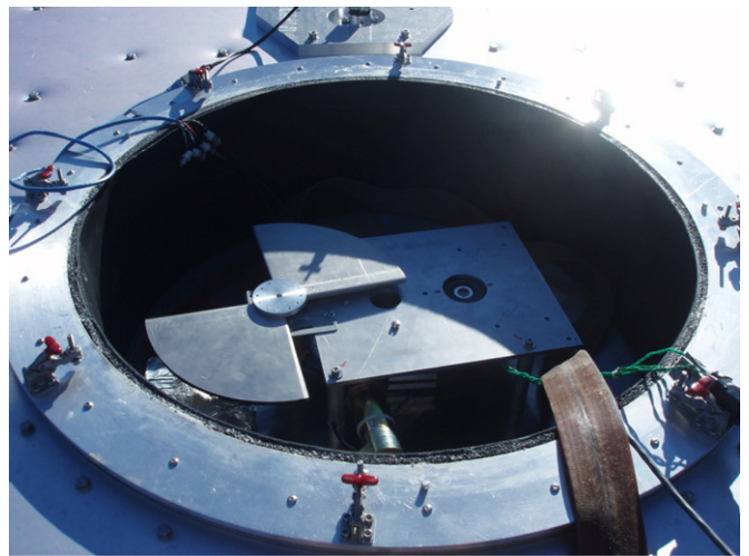
Figure 13. Device above the cryostat window for measuring cross-polarization responses and PSB orientations. The window is covered with a metal plate with a 2 \text{ cm} Eccosorb aperture, and a 10 \text{ cm} diameter wire grid is on a rotation stage under the circular aperture of the rectangular plate. The chopper modulates the load between the ambient temperature and the cold sky.
