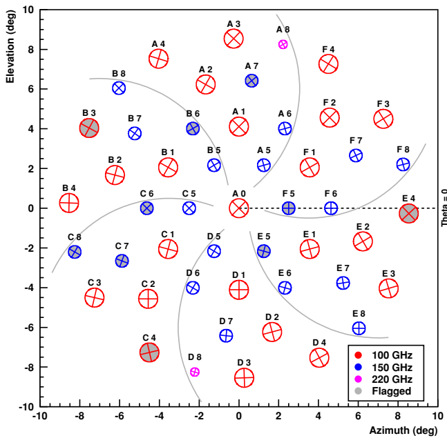
Figure 2. 2007/2008 layout of the BICEP beams with nominal locations, FWHM, and polarization orientations. There are six sections (separated by curved gray lines) having alternating “Q” or “U” PSB orientations with respect to the center. The observations are performed with the focal plane orientations of -45^\circ , 0^\circ , 135^\circ , and 180^\circ counterclockwise about the boresight, providing two independent and complete polarization coverages of the field to allow jackknife tests. (A 180^\circ boresight rotation provides complete coverage of Q and U Stokes parameters on the sky at each beam location.)
