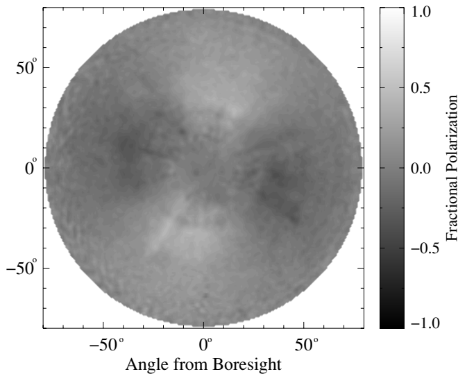
Figure 16. Map of fractional polarization for a 100 GHz feed (“C1”) up to 80^\circ from the beam center, showing the gain-adjusted pair difference divided by the pair sum. Beyond \sim 15^\circ from the boresight where the forebaffle cuts off the beam, the sidelobes are generally up to 50% polarized, but with smooth quadrupole pattern aligned with the polarization sensitivity.
