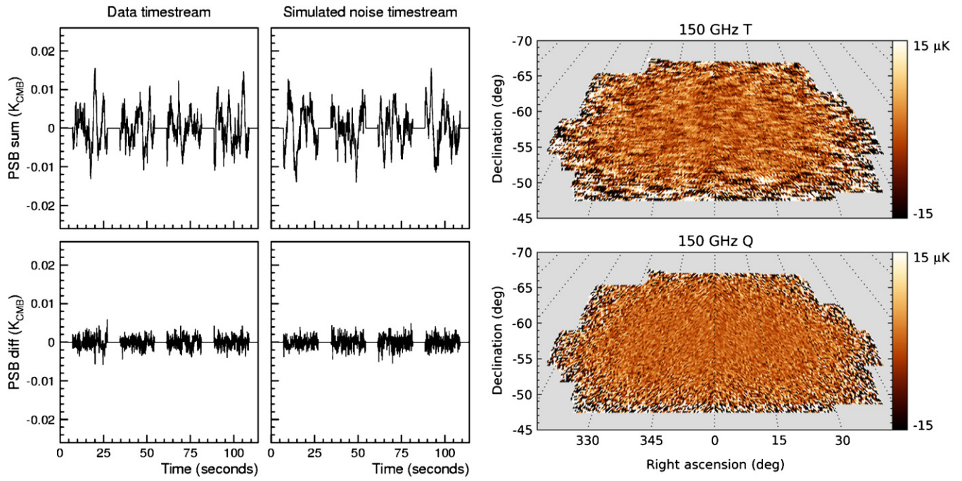
Figure 21. Real and simulated-noise timestreams for a PSB pair over four azimuth half-scans, showing that the noise qualities are accurately reproduced. The simulated timestreams for all the PSB pairs over the two years are co-added to form the noise-only maps (right). The 1/f noise causes striping in the T map, while the Q polarization map approximates white noise.
