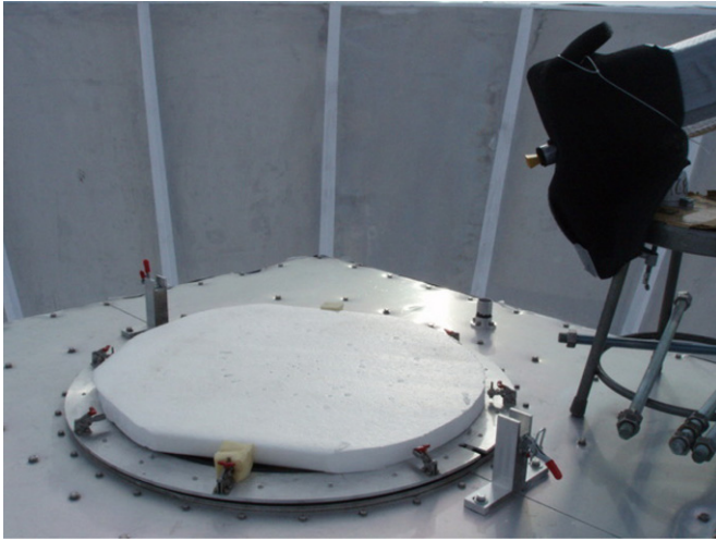
Figure 4. Modulated source in front of the telescope aperture used for the measurement of transfer functions. Metal washers are embedded in transparent polypropylene foam sheet to scatter the PIN-switched broadband noise source signal (from upper right) into the beam while keeping the total loading similar to that during nominal CMB observations.
