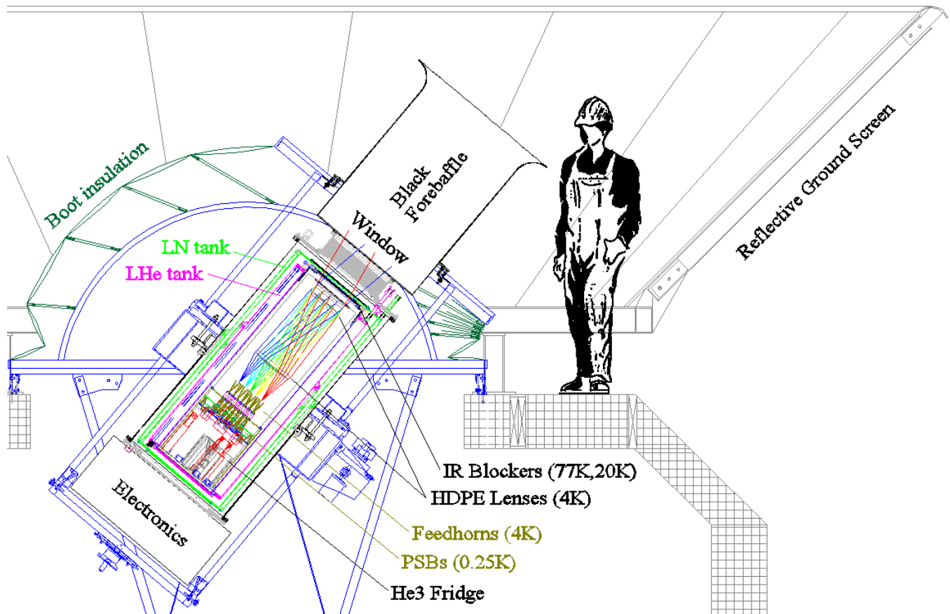
Figure 1. BICEP telescope on a three-axis mount at its lowest elevation limit of 50^\circ , looking out through the roof of the Dark Sector Laboratory (DSL) building located 800 m from the geographic South Pole. A cryostat with toroidal liquid nitrogen and liquid helium tanks encloses the entire 4 K optics, including two high-density polyethylene lenses and corrugated feedhorns. The PSBs are cooled with a ^4\text{He}/^3\text{He}/^3\text{He} sorption refrigerator to 250 mK.
