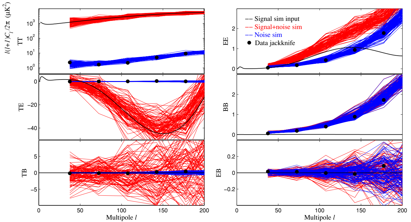
Figure 22. 150 GHz power spectra of 100 realizations of simulated signal+noise and noise only, compared to the scan-direction jackknife spectra from the actual data. The distributions of simulated noise spectra are consistent with the data jackknife spectra, which are expected to be signal-free and a good representation of noise in the data. The CMB signal simulation uses the input spectra shown. Error bars in the final spectra are determined by the scatter in the signal+noise spectra, which is noise-dominated for BB and EB and largely cosmic variance limited for other spectra.
