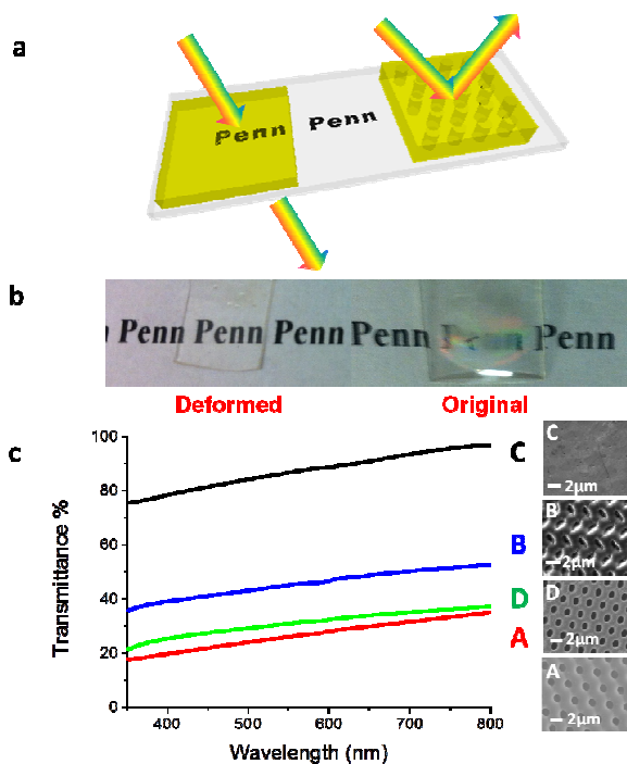
Fig. 3 Display of “Penn” logos underneath 2D SMP membranes. a. Schematic illustration of transparency comparison between the deformed and the original SMP membranes. b. Optical images of the deformed and original SMP membranes on top of the “Penn” logo. The “Penn” underneath the original membrane is hardly legible but clearly visible under the deformed sample. c. UV-Vis spectra of different 2D SMP membranes (A-D) using the bulk SMP film as a reference. A. Original. B. Deformed at \varepsilon \sim 13 \pm 2\% . C. Deformed at \varepsilon \sim 30 \pm 2\% . D. Recovered one.
