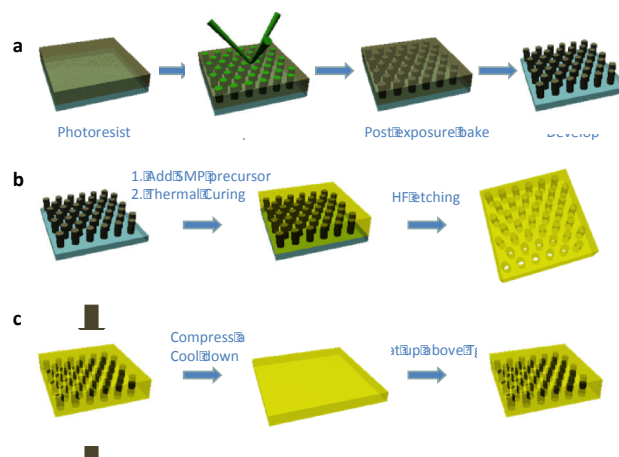
Fig.1 Schematic illustration of fabrication and deformation/recovery of a 2D SMP membrane. (a) Fabrication of 2D pillar array by holographic lithography. (b) Fabrication of SMP membrane with periodic holes by replica molding, followed by etching in HF aqueous solution. (c) Hot-pressing of SMP membrane in the vertical direction above T_g . The temporary shape could be fixed by cooling down to room temperature under the load. The original shape could be recovered upon reheating above T_g .
