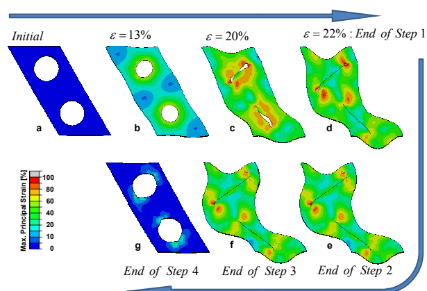
Fig. 4 Numerical results for the SMP thermo-mechanical cycle. Snapshots of the hexagonal lattice during Step 1, hot-pressing at different strain levels (a-d), and at the end of Steps 2, cooling down (e), 3, un-loading (f) and 4, reheating (g). The color gives indications of the maximum principal strain distribution.
