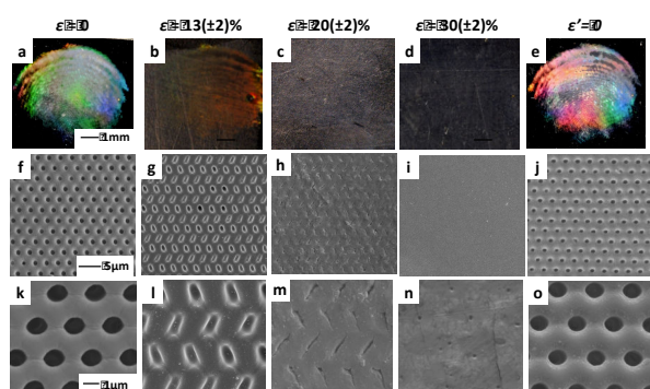
Fig. 2 Pattern transformation and recovery in a 2D SMP membrane. (a-e) Optical images of the (a) original, (b-c) partially deformed, \varepsilon \sim 13 \pm 2\% (b) and \varepsilon \sim 20 \pm 2\% (c), (d) completely deformed, \varepsilon \sim 30 \pm 2\% , and (e) recovered SMP membranes. (f-j) Corresponding SEM images of the SMP membranes shown in (a-e). (k-o) Higher magnification SEM images of (f-j).
