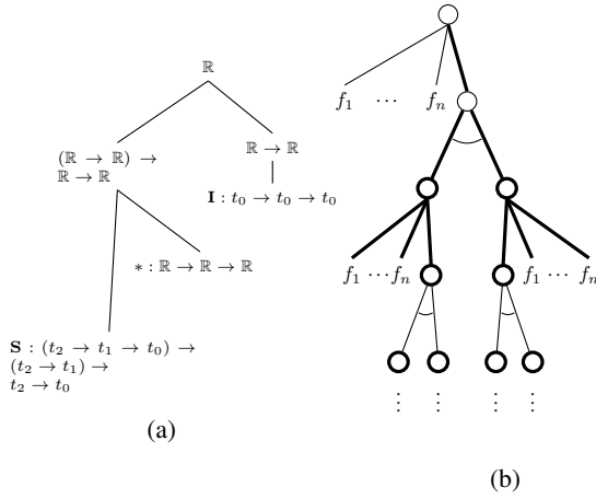
Figure 1: (a) The typed combinator S * I (f(x) = x^2 over real values ( \mathbb{R} )) represented as a binary tree. (b) The space of all typed combinators represented as an infinitely deep AND/OR tree.
