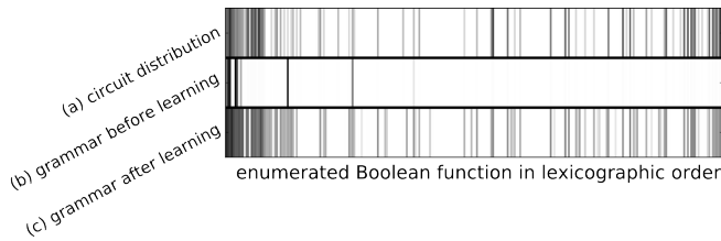
Figure 5: Distribution of Boolean functions among (a) the set of 1000 circuits randomly constructed from AND, OR and NOT gates (see text); b) the first 1000 expressions from the grammar over expressions before learning; c) the first 1000 expressions from the grammar over expressions after learning. Gray levels indicate percent of instances (circuits/expressions) which evaluate to that function. Functions increase in domain size from left to right; each function can be represented as a binary string corresponding to the output column of the truth table, and functions are ordered with respect to these strings.
