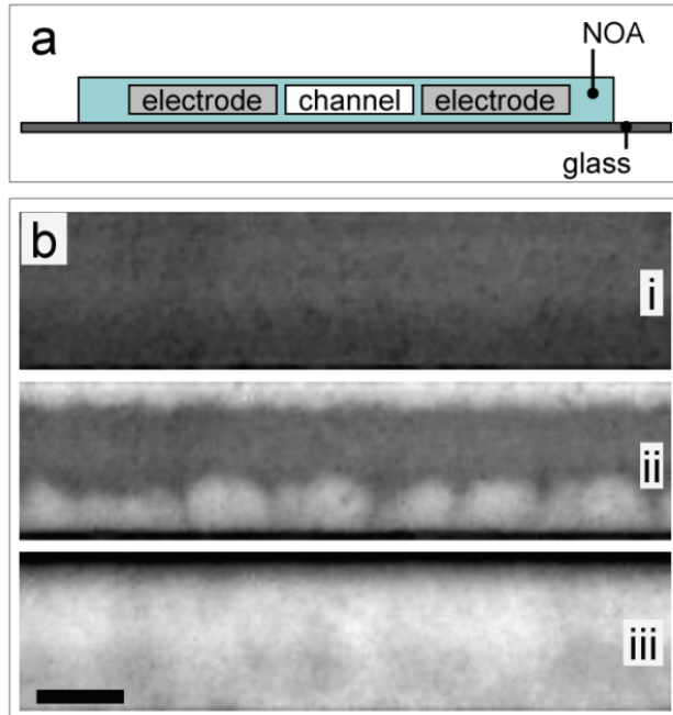
Figure 4.1: (a) Cross-sectional schematic of microfluidic device. (b) Top view of a channel containing carbon black particles. The particles are initially distributed homogeneously within the channel in the absence of an applied field (i), partially transported to the bottom wall when a field of magnitude 2 \text{ V}/\mu\text{m} is first applied across the channel (ii), and completely packed at the top wall when the direction of the field is switched (iii). The particles are transported completely across the channel and packed at the wall after all subsequent switches. Scale bar is 25 \mu\text{m} .
