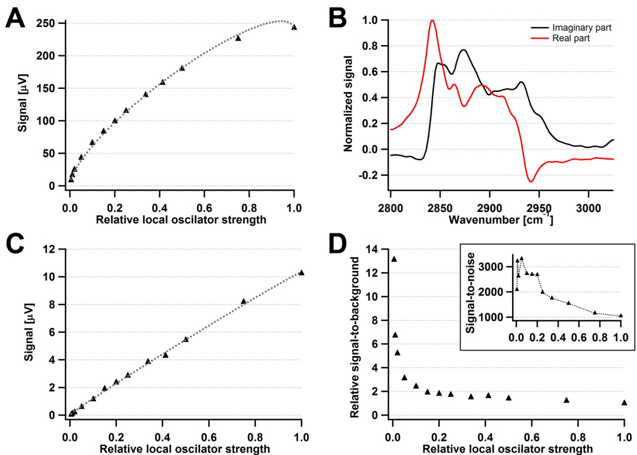
Figure 4. OHD-RIKE micro-spectroscopy. (A) OHD-RIKE signal of methanol at 2830\text{cm}^{-1} as a function of the local oscillator strength relative to the total pump beam intensity. Dashed linear is the fit with equation (6). (B) OHD-RIKE spectra of dodecane with the phase of local oscillator set to probe the real (red line) and imaginary part (black line) of the non-linear susceptibility tensor. (C) Cross phase modulation of water at 2930\text{ cm}^{-1} as a function of the local oscillator strength. Dashed linear is the fit with equation (6). (D) Ratio of methanol signal (shown in A) to cross phase modulation background (shown in C) normalized to by the signal from pure SRS. Inset: signal-to noise-ratio of the signal of pure methanol (shown in A) over the noise of the cross phase modulation signal in C.
