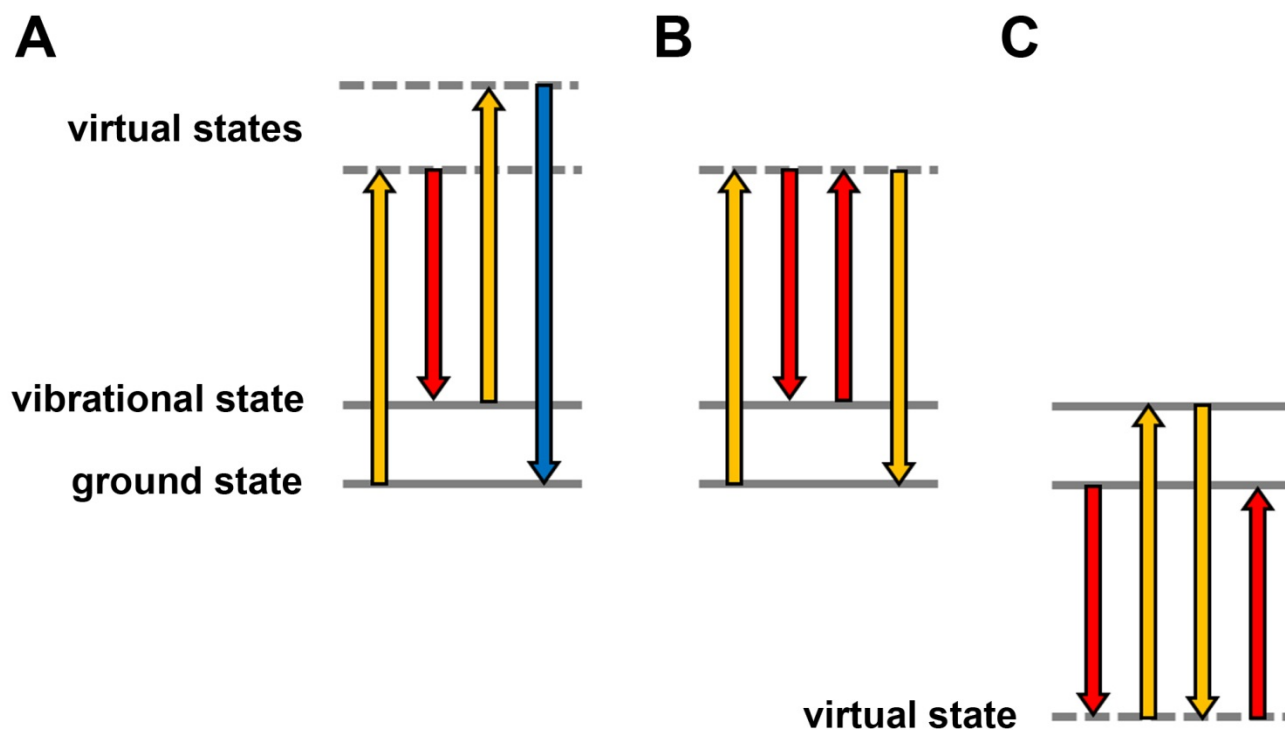
Figure 1. Coherent Raman Scattering techniques. Energy diagrams of (A) CARS, (B) SRL and RIKE of the pump beam and (C) SRG and RIKE of the Stokes beam. All processes probe the vibrational excited state of the molecules in focus. Virtual states originate from the electronic response, are instantaneous and thus can have an undefined energy different from the Eigen states of the system (even negative as in (C)). Different directions of the emission light indicate different phase relationships with the excitation beams.
