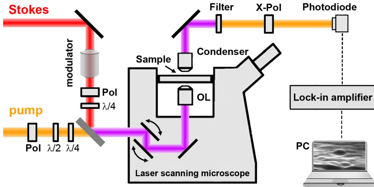
Figure 3. Experimental setup for circular OHD-RIKE microscopy. Pump and Stokes beam are provided by a mode-locked Nd:YVO 4 laser at 1064nm (Stokes beam), which synchronously pumps an optical parametric oscillator with tunable output from 650nm to 1020nm (pump beam). The amplitude of the Stokes beam is modulated with a resonant Pockels cell, spatially overlapped with the pump beam with a dichroic mirror (DM) and aligned into a laser scanning microscope. Collinear beams are focused by the objective lens (OL) into the sample. Transmitted beams are collected with a condenser. After blocking the Stokes beam with a filter, the intensity of the pump beam is detected with a photodiode. A lock-in amplifier measures the amplitude of the modulation transfer to the pump beam due to the non-linear interaction with the sample to provide the intensity of a pixel. For OHD-RIKE, the pump and Stokes beams are first linearly polarized with polarizers (Pol) and a cross-polarizer (X-Pol) is inserted in front of the photodiode to block the transmitted pump beam. The exact position is set by the intensity dependence after a polarizer. For circular RIKE, the Stokes beam is circular polarized with a quarter-wave plate ( \lambda/4 ), which would be replaced by a half-wave plate for linear RIKE. For OHD-RIKE, we install a half-wave plate ( \lambda/2 ) in the pump beam path to adjust the amount of transmitted light through the cross-polarizer in order to control the strength of the local oscillator. The phase of the local oscillator can be shifted by 90° to selectively probe imaginary part of the non-linear response by a quarter wave plate ( \lambda/4 ) in the pump path along the axis of the local oscillator.
