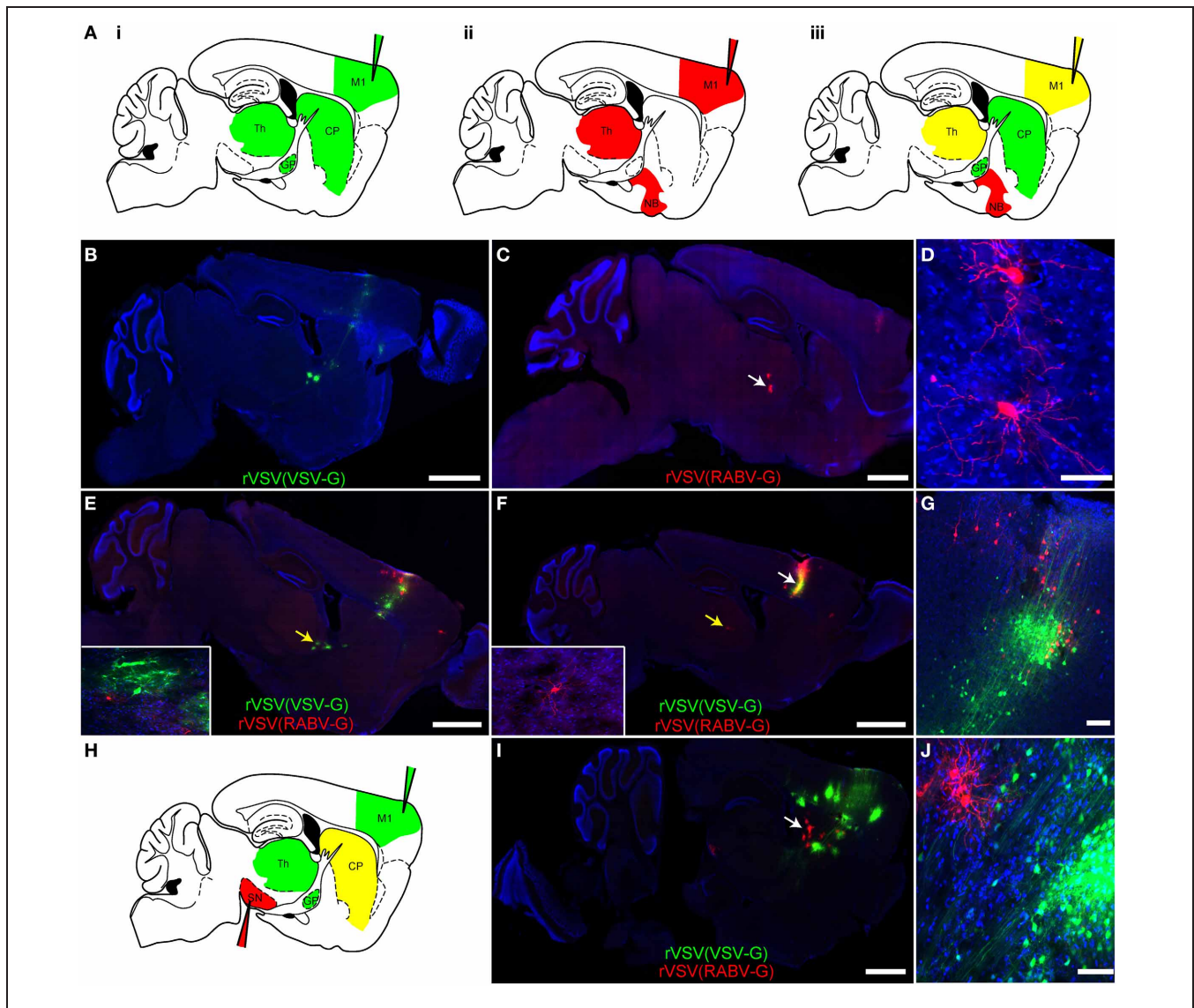
FIGURE 6 | Simultaneous anterograde and retrograde transsynaptic circuit tracing using rVSV. (A) Connectivity schematics of parasagittal sections indicating patterns of spread from injection of M1 (injection needles) with a polysynaptic virus transmitting across synapses in the (i) anterograde or (ii) retrograde directions. Panel (iii) shows the pattern from co-injection of two polysynaptic viruses, one anterograde and one retrograde. Green represents the anterograde virus, red the retrograde virus, and yellow, both. Note that yellow indicates that the area is predicted to host infection by both viruses, with potentially some individual cells showing infection with both viruses. (B) The anterograde transsynaptic virus rVSV(VSV-G), when injected alone, labeled M1 as well as anterograde projection areas, such as the CP, GP, and thalamus, whereas (C) the retrograde virus rVSV(RABV-G) labeled M1 as well as areas projecting to the cortex, including the thalamus. (D) High magnification of thalamic cells shown in (C) (white arrow). (E,F) Examples taken from a series of parasagittal sections from the same brain of an animal injected with both viruses simultaneously into M1. Co-infection of cells in M1
