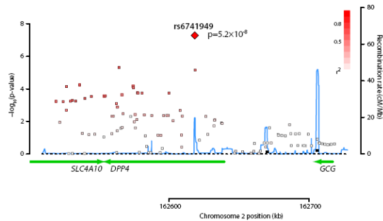
Figure 2. Regional plots for hippocampal volume SNPs
