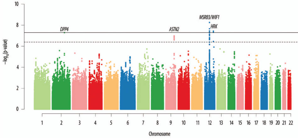
Figure 1. Genome-wide Manhattan plot for hippocampal volume The plot shows the individual p-values (based on discovery meta-analysis) against their genomic position for hippocampal volume. Within each chromosome, shown on the x-axis, the results are plotted left to right from the p-terminal end. The dashed line indicates the threshold for follow-up, p < 4 \times 10^{-7} and the solid line indicates the threshold for genome-wide significance, p < 5 \times 10^{-8} . The nearest genes are indicated above points that surpassed our significance threshold for follow-up.
