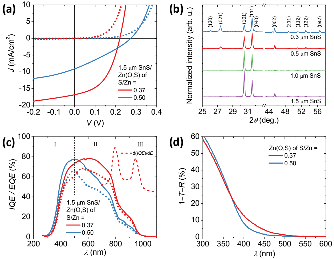
FIG. 3. (a) J - V characteristic of 1.5 \mu m-thick SnS devices with \text{Zn(O,S) of S/Zn} = 0.37 and 0.50 under dark (dotted line) and approximately 1 sun illumination (solid line). (b) XRD spectra of SnS at the film thicknesses of 0.3, 0.5, 1.0, and 1.5 \mu m. The intensity was normalized by the (111) peak. (c) IQE (solid line) and EQE (dotted line) of the same devices. The peaks of the IQE derivatives in the \text{S/Zn} = 0.37 device correspond to the strong absorption edges of SnS at 1.32 and 1.55 eV. (d) Effective absorption ( 1 - T - R ) of 60 nm-thick \text{Zn(O,S) of S/Zn} = 0.37 and 0.50 .
