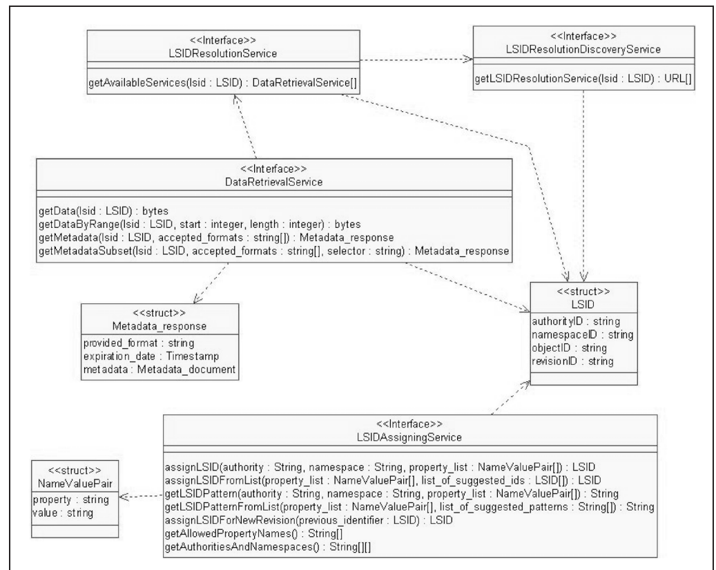
Figure 1: UML diagram showing LSID/LSRS components and their relationships Adapted from EMBL-EBI, I3C, IBM 34
