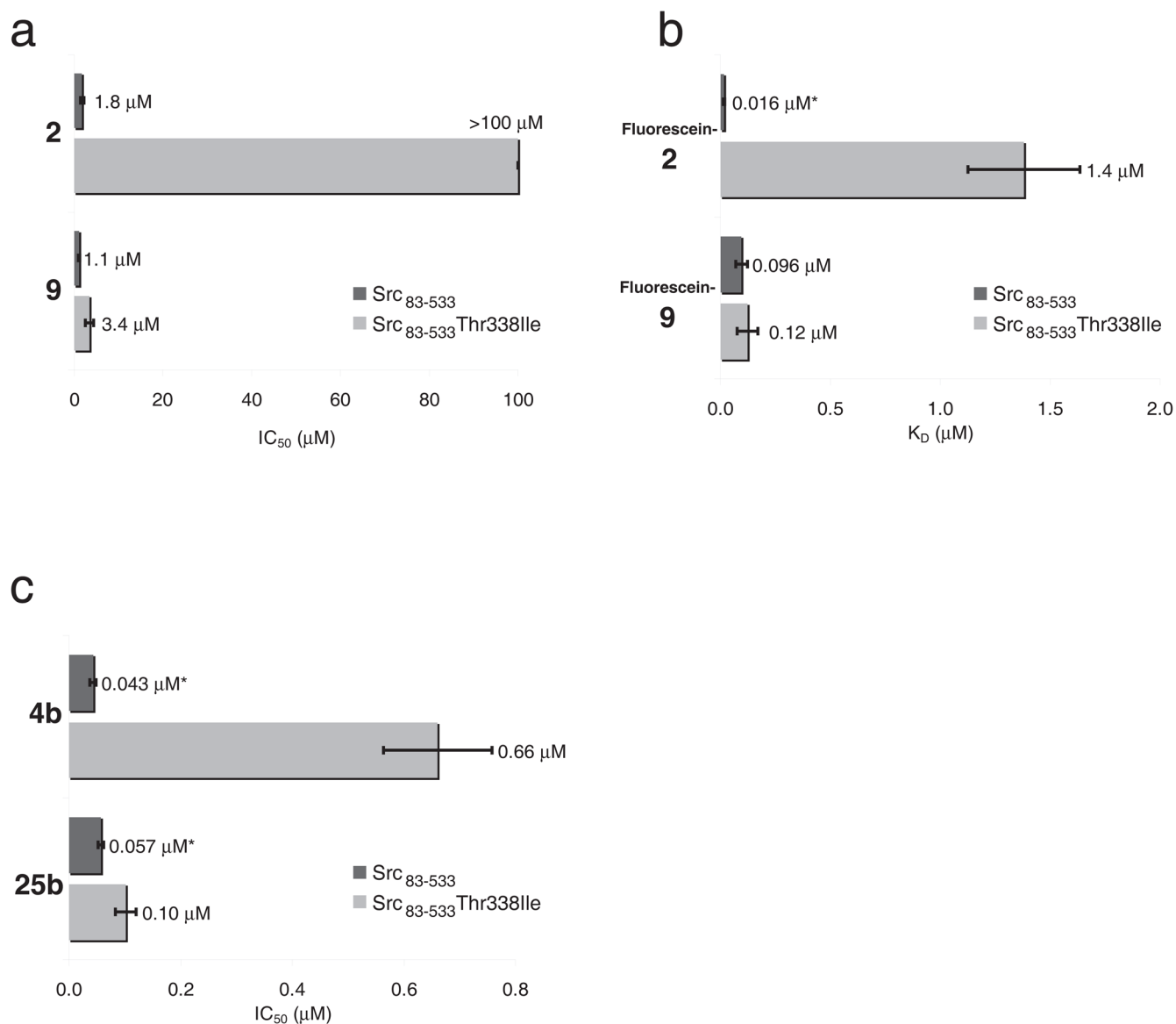
Figure 6. Activity of the macrocycles against the Thr338Ile gatekeeper mutant of Src kinase. (a) IC 50 of 2 , and 9 for Src 83-533 and Src 83-533 T338I. IC 50 values for 2 and 9 were determined in the presence of 5 μM ATP, 100 μM Src-optimal peptide. (b) Measurement of the dissociation constant K D of fluorescein-labeled 2 and 9 for Src 83-533 and Src 83-533 T338I. *Value is an upper estimate of the K D because the K D is lower than the concentration of macrocycle compound used in the assay. (c) IC 50 of 4b , and 25b for Src 83-533 , and Src 83-533 T338I. IC 50 values for 4b and 25b were determined in the presence of 250 μM ATP and 300 μM Src-optimal peptide. *Values are an upper estimate of the IC 50 because the apparent IC 50 is lower than the concentration of kinase used in the assay. All experiments were performed in triplicate, and data represent mean values ± standard deviation.
