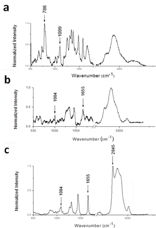
Figure 2. Raman spectra of (a) DNA, (b) BSA and (c) Oleic Acid
