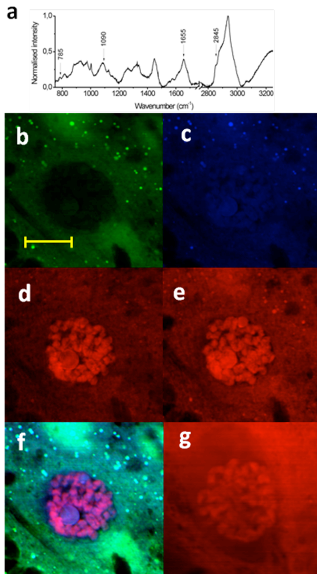
Figure 3. (a) Raman spectrum of a Drosophila cell (b)-(g) SRS images of a salivary gland cell from Drosophila melanogaster , via the stimulated Raman loss detection scheme. (b) Lipid specific image taken at 2845\text{cm}^{-1} , (c) Amide I band at 1655\text{cm}^{-1} (d) nucleic acids at 785\text{cm}^{-1} and (e) 1090\text{cm}^{-1} . (f) multicolor image generated by combining images (b)-(e). (g) Nucleic acid map recorded at 785\text{cm}^{-1} via the stimulated Raman gain detection scheme. Scale bar is 20\text{ }\mu\text{m} . Each image has a size of 512 \times 512 pixels.
