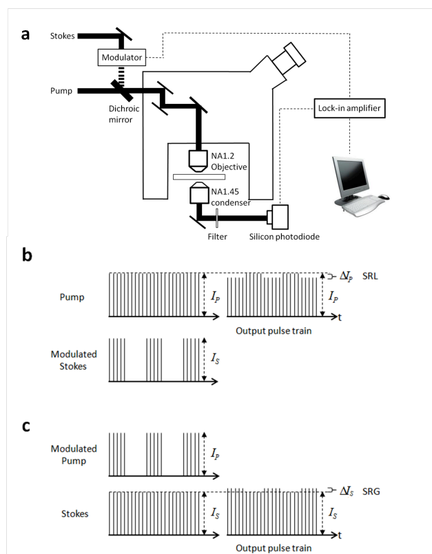
Figure 1. (a) Experimental schematic of stimulated Raman loss (SRL) microscope. For SRG, the pump beam is modulated instead of the Stokes beam and an InGaAs photodetector is used instead of a silicon photodetector because of its better responsivity at 1064 nm. (b) Detection scheme of SRL. Stokes beam is modulated at 10.4 MHz at which the resulting amplitude modulation of the pump beam due to the stimulated Raman loss can be detected. (c) Detection scheme of SRG. Pump beam is modulated at 10.4 MHz at which the resulting amplitude modulation of the Stokes beam due to the stimulated Raman gain can be detected.
