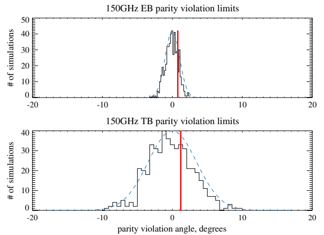
FIG. 1 (color). \Delta\alpha measured from QUaD 150 GHz TB and EB spectra; histogram of simulations and red line for data. The histogram does not account for systematic error. The dotted line indicates total uncertainty assuming a Gaussian 0.5^\circ systematic error.
