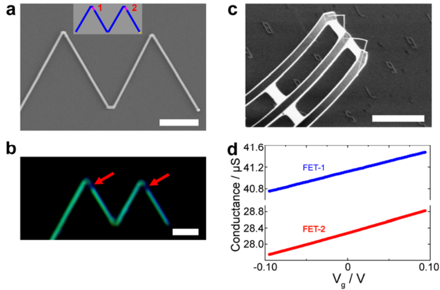
Figure 4. Parallel nanoFET KNWs. a , SEM image of a W-shaped parallel-nanoFET KNW. Scale bar, 2 μm. Inset: Schematic of the W-shaped KNW with one nanoFET encoded at the tip of each V-shaped component of the “W”, where blue and pink indicate heavily-doped connections and lightly-doped nanoFET channels, respectively. b , Dark-field optical microscopy image of KOH etched W-shaped KNW. The two dark color segments correspond to the lightly doped nanoFET elements (red arrows) near the two tips. Scale bar, 2 μm. c , SEM image of W-shaped parallel-nanoFET KNW bend-up probe. Scale bar, 20 μm. d , Conductance versus water-gate reference potential data recorded independently from two parallel nanoFETs.
