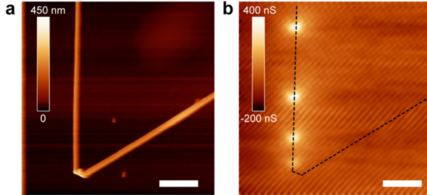
Figure S2. Scanned probe microscopy characterization of a multi-nanoFET KNW. (a) AFM image of series multi-nanoFET KNW. Scale bar, 2 \mu\text{m} . Color scale (0 to 450 nm) corresponds to the z-height of the image; the KNW is \sim 150 nm in diameter. (b) Corresponding SGM image of the multi-nanoFET KNW with V_{\text{tip}} of +10 V. Scale bar, 2 \mu\text{m} . The bright regions in SGM image correspond to increased NW conductance. Color scale (-200 to 400 nS) corresponds to the conductance change. SGM measurements were made as described in reference-38 using a S/D voltage of 0.1 V.
