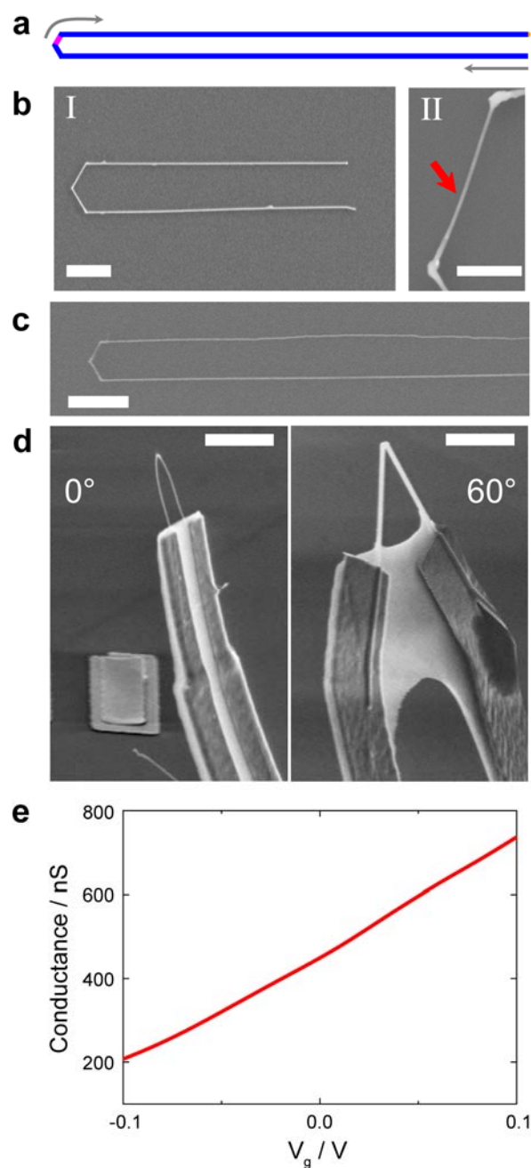
Figure 2. U-shaped KNWs. a , Schematic of a U-shaped KNW with tip constructed from three 120^\circ cis -linked kinks. The lightly-doped n-type nanoFET element (pink) is encoded at the tip and connected by heavily-doped n^{++} S/D arms (blue). The grey arrows indicate the growth sequence for the nanostructure. (b) SEM images of original (I: scale bare, 2 \mu m) and KOH-etched (II: scale bar, 500 nm) U-shaped KNW synthesized with 80 nm diameter Au-NP catalysts. Red arrow marks the position of nanoFET element between the second and the third cis -linked kinks. c , Representative SEM image of a
