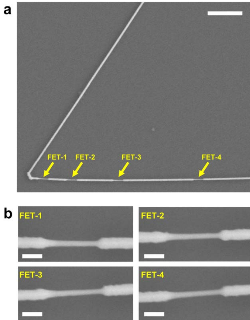
Figure S1. Series multi-nanoFET functional KNW. (a) Representative SEM image of a KOH-etched series multi-nanoFET KNW. The segments with smaller diameter correspond to preferentially-etched lightly-doped nanoFET elements. Scale bar, 2 \mu\text{m} . (b) Magnified images of the 4 nanoFET elements marked with arrows in a . Scale bars, 200 nm. Series multi-nanoFET KNWs were dispersed from ethanol solutions onto the nitride surface of Si/SiO 2 /Si 3 N 4 substrates (NOVA Electronic Materials Inc.), and then etched in KOH solution to highlight the lightly-doped nanoFET sections (see reference-34, manuscript).
