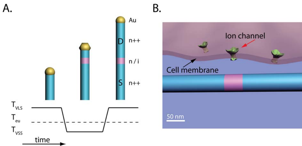
Figure 1. Overview of the synthesis and cellular interfaces of short channel NWFETs. (A) Illustration of Au nanoparticle catalyzed NW growth with well-controlled axial dopant profile introduced during VSS growth. Initially a n^{++} S electrode is synthesized via the VLS mechanism. Subsequently, either n or i active device regions are encoded by VSS growth. Lastly, another VLS phase of growth completes the n^{++} D electrode. (B) Schematic of a short-channel NWFET interfaced with an extracellular region of an electrogenic cell.
