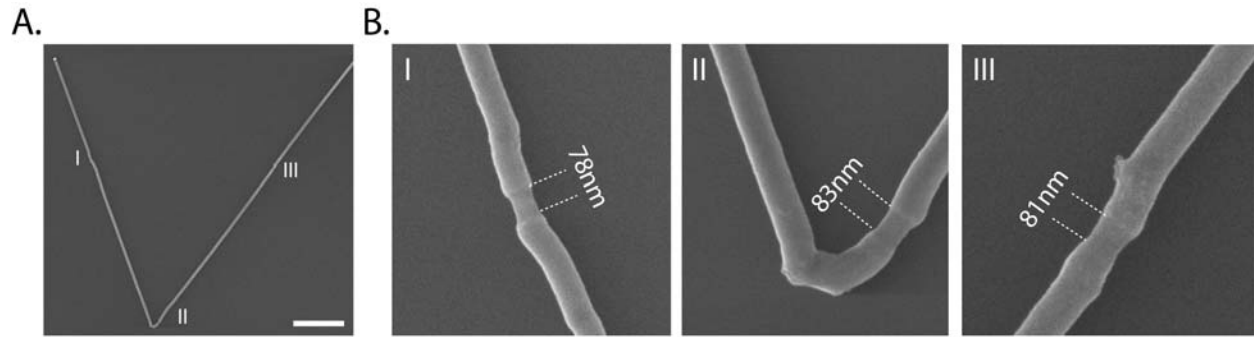
Figure S1. Multiple short channel NWs synthesized on a single Si NW. A. SEM image of a representative 80 nm Si NW with three 80 nm channel length devices. Scale bar is 1.5 \mu\text{m} . B. An expanded view of the short channel segments marked as I, II and III. Synthesized SiNWs were dispersed from isopropanol solutions onto the nitride surface of Si/SiO 2 /Si 3 N 4 substrates (NOVA Electronic Materials Inc.), then KOH selective etching was used to highlight the transition between n ++ to intrinsic sections. 10gr of KOH (Sigma-Aldrich Inc.) were dissolved in 88mL DI H 2 O and 37mL isopropanol. Substrates with dispersed NWs were dipped in the solution for 3-8sec at 50°C-60°C. The substrates were rinsed with DI H 2 O, followed with isopropanol rinse and dried in a N 2 stream.
