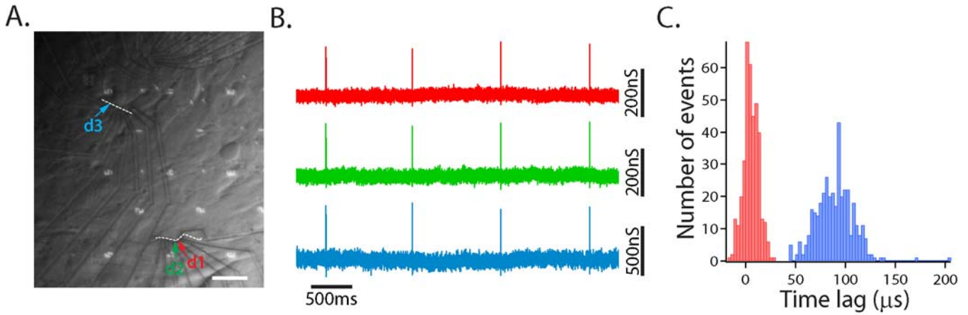
Figure 5. Recording from short-channel SiNW FETs on multiple length scales. . (A) Optical image of cardiomyocytes interfaced with three 130 nm channel length devices (labeled d1, d2, and d3). White dashed lines illustrate the NW position; scale bar is 15 \mu\text{m} . (B) Representative recorded signals from d1 (red), d2 (green), and d3 (blue). (C) Histogram of the time lag between devices d1 and d2 (red; separation distance 1.9 \mu\text{m} ) and between devices d1 and d3 (blue; separation distance 73 \mu\text{m} ).
