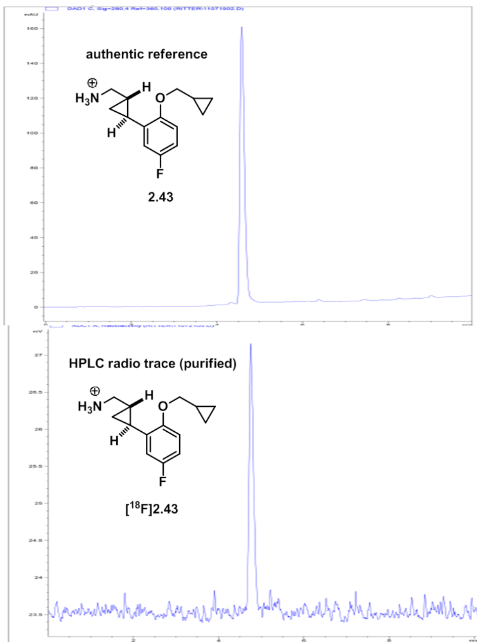
Figure 4.17. Characterization of purified [ 18 F]2.43. Note: radioactivity chromatographs have been not been offset (-0.125 min) to account for the delay volume (time) between the diode array detector and the radioactivity detector.
