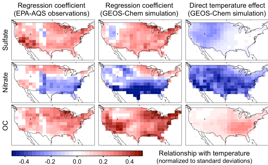
Figure 3.3. Relationships of sulfate, nitrate, and organic carbon (OC) PM_{2.5} concentrations with surface air temperature. The left and middle panels show the observed (2004-2008) and simulated (2005-2007) standardized regression coefficients \beta_1 in Eq. (3.1). Values are for deseasonalized and detrended variables and are only shown when significant with 95% confidence ( p -value < 0.05 ). The right panels show the direct effects of temperature on sulfate, nitrate and OC as determined by applying a global +1 K temperature perturbation in the GEOS-Chem simulation, and normalizing the results to the standard deviations of deseasonalized concentrations and temperatures to allow direct comparison to \beta_1 .
