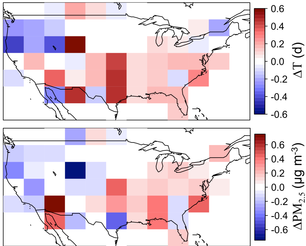
Figure 4.6. Projected 2000-2050 changes in the periods of the dominant meteorological modes for PM_{2.5} variability (top), and implied changes in annual mean PM_{2.5} (bottom). The changes in synoptic periods ( \Delta T ) are weighted averages from the ensemble of IPCC AR4 GCMs calculated using the Bayesian-REA approach of Tebaldi et al. (2004, 2005). The implied changes in PM_{2.5} ( \Delta PM_{2.5} ) are calculated as \Delta PM_{2.5} = (dPM_{2.5}/dT)\Delta T where dPM_{2.5}/dT is the local relationship from Fig. 4.2. When two or more meteorological modes have similar correlation with annual PM_{2.5} , an average effect from these modes is calculated.
