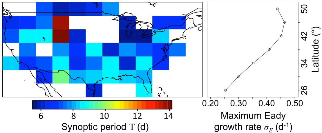
Figure 4.3. Mean synoptic periods T of the dominant meteorological modes for interannual PM_{2.5} variability in NCEP/NCAR Reanalysis 1 observations for 1981-2000. Also shown is the latitudinal profile of maximum Eady growth rate \sigma_E as calculated by Eq. (4.2) for 0^\circ - 180^\circ W and 850-500 hPa.
