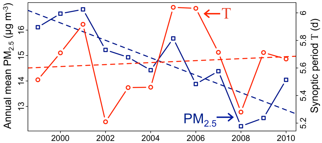
Figure 4.1. Observed 1999-2010 time series of annual mean PM_{2.5} and synoptic period T of the dominant meteorological mode (cold frontal passage) for the 4^\circ \times 5^\circ grid square centered over Chicago at N42^\circ W87.5^\circ (asterisk in Fig. 4.2). Linear regression lines are shown as dashed. The detrended variables have a correlation of r = 0.62 .
