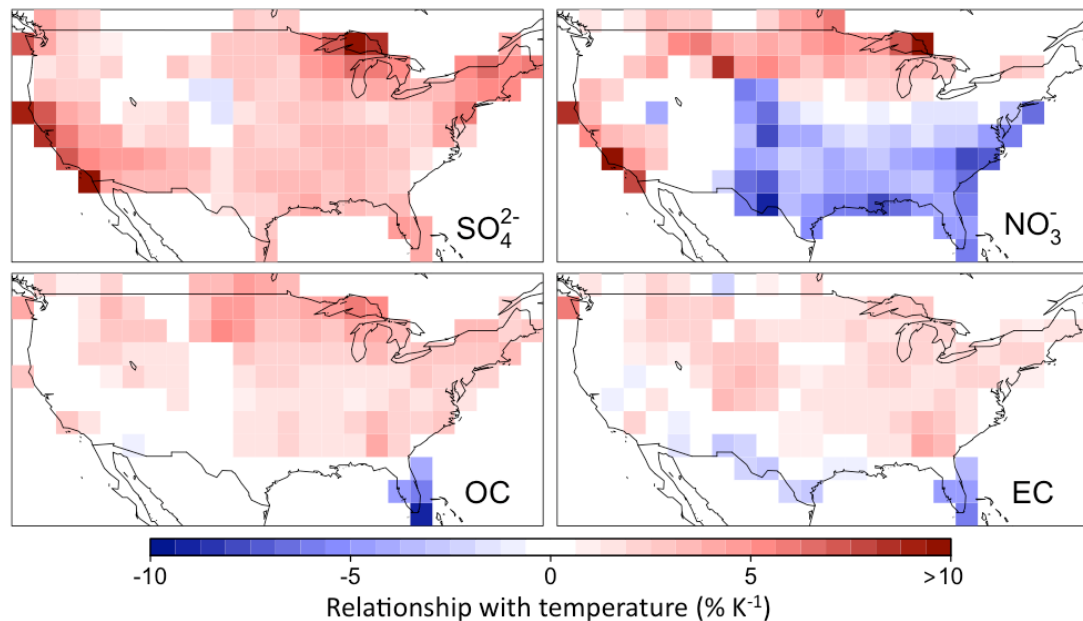
Figure 2.7. Correlations of PM 2.5 components with surface air temperature. Figure shows multiple linear regression coefficients \beta_1 , normalized to annual mean concentrations of Fig. 2.3. Values are for deseasonalized and detrended variables and are only shown when significant with 95% confidence ( p -value < 0.05).
