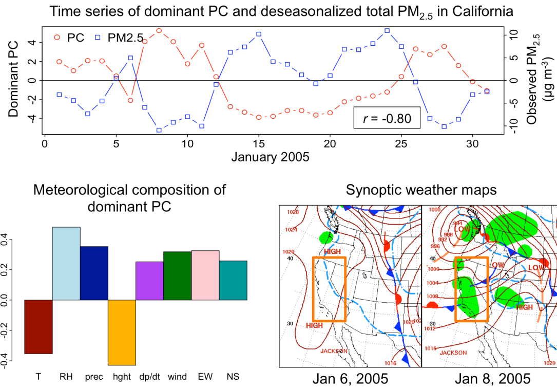
Figure 3.7. Same as Fig. 3.6 but for California.
