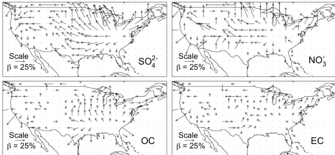
Figure 2.9. Correlations of PM 2.5 components with wind direction. Figure shows vector sums of multiple linear regression coefficients \beta_8 and \beta_9 , normalized to annual mean concentrations of Fig. 2.3. Length of arrows (in units of % per unit sine or cosine) indicates magnitude of correlation. Values are for deseasonalized and detrended variables and are only shown when significant with 95% confidence ( p -value < 0.05).
