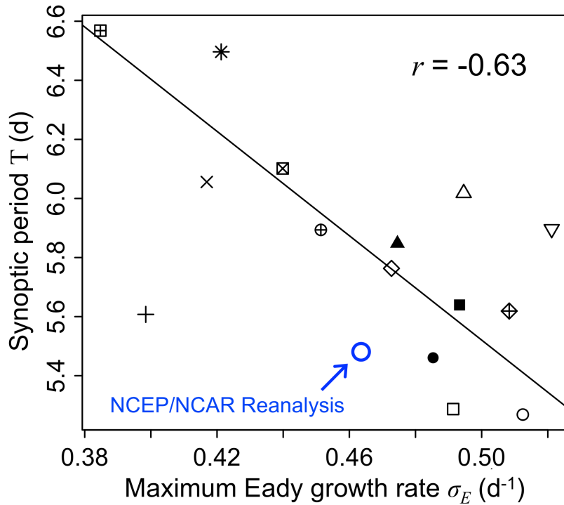
Figure 4.5. Relationship between atmospheric baroclinicity and synoptic period T of the dominant meteorological mode for PM_{2.5} variability in the Chicago grid cell as simulated by 15 IPCC AR4 GCMs for 1981-2000. The observed value from the NCEP/NCAR Reanalysis 1 is also indicated. Baroclinicity is measured as the maximum Eady growth rate \sigma_E for 44^{\circ} - 48^{\circ} N and 850-500 hPa. Each symbol represents an individual GCM (see Fig. 4.4). Correlation coefficient and reduced-major-axis regression slope are also shown.
