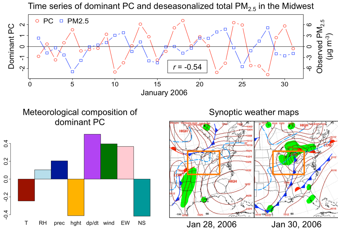
Figure 3.6. Dominant meteorological mode for observed PM_{2.5} variability in the Midwest inferred from the principal component analysis. Top panel: time series of deseasonalized observed total PM_{2.5} concentrations and the dominant meteorological mode or principal component (PC) in January 2006. Bottom left: composition of this dominant mode as measured by the coefficients \alpha_{ki} in Eq. (3.3). Meteorological variables ( x_k ) are listed in Table 3.1. Bottom right: synoptic weather maps from NCEP ( http://www.hpc.ncep.noaa.gov/dailywxmap/ ) for 28 and 30 January, corresponding to maximum negative and positive influences from the principal component. The Midwest is delineated in orange.
