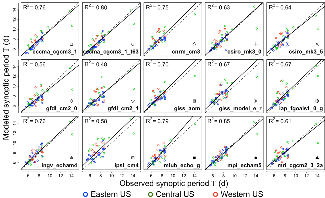
Figure 4.4. Scatterplots of modeled vs. observed synoptic periods T of dominant meteorological modes for interannual PM_{2.5} variability in the US for 1981-2000. Observed values are from NCEP/NCAR Reanalysis 1, and modeled values from 15 IPCC AR4 GCMs. GCM names are given in each panel, and the symbol above each name is used to identify the model in Fig. 4.5 and 4.7. Each data point represents T for one 4^\circ \times 5^\circ grid cell, and the ensemble of points represents the continental US separated as eastern (east of 95^\circ W ), central ( 110^\circ - 95^\circ W ), and western (west of 110^\circ W ). The solid black line is the reduced major-axis regression slope, with coefficient of variation ( R^2 ) also given. The 1:1 line is shown as dashed.
