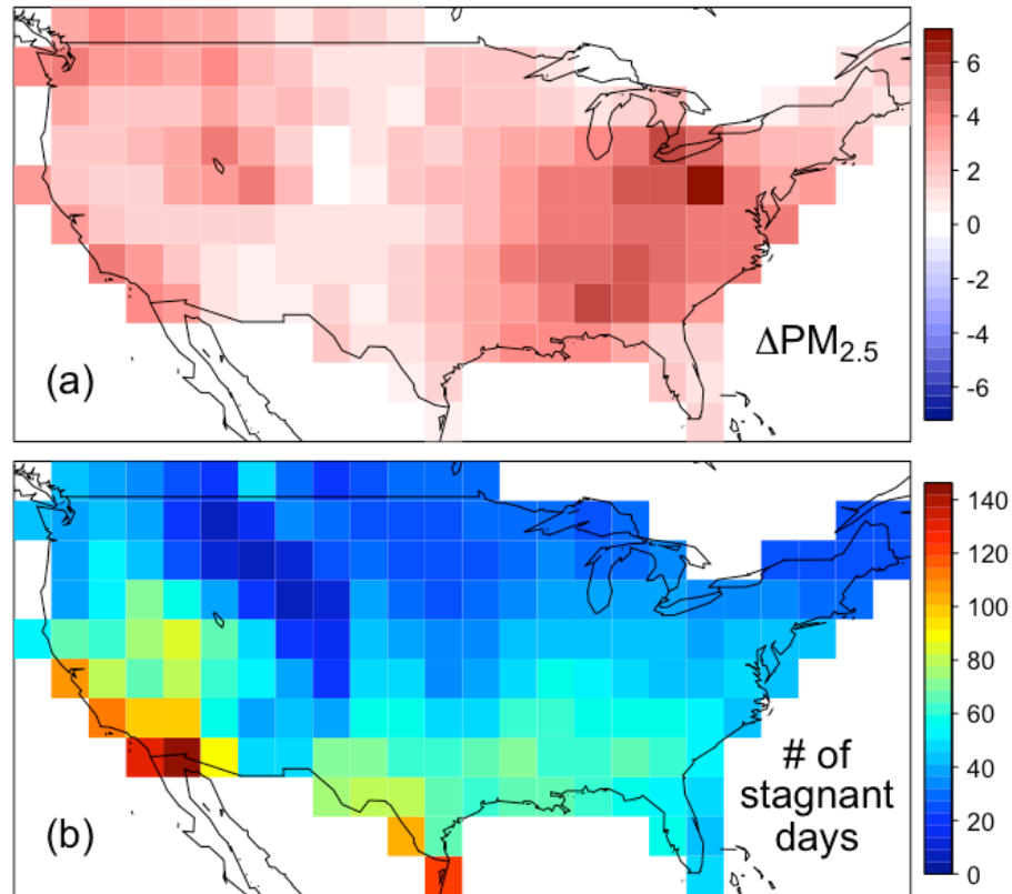
Figure 2.6. (a) Average differences in deseasonalized total PM 2.5 concentrations on stagnant vs. non-stagnant days, based on deseasonalized and detrended 1998-2008 observations. Stagnation is defined following Wang and Angell (1999). Only differences with 95% confidence ( p -value < 0.05) are shown. (b) Number of stagnant days per year averaged over 1998-2008.
