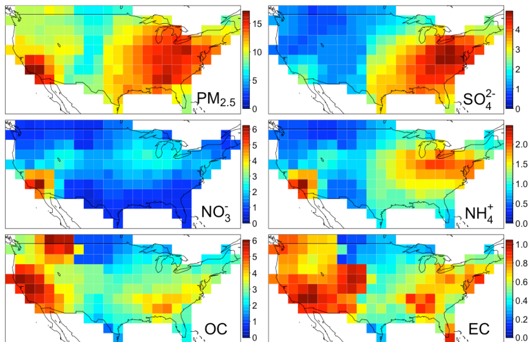
Figure 2.3. Annual mean concentrations of total PM_{2.5} and its five major components, interpolated on a 2.5^\circ \times 2.5^\circ grid as described in text. Concentrations are in units of \mu\text{g m}^{-3} and averaged over 1998-2008 for total PM_{2.5} and 2000-2008 for individual species. OC concentrations were adjusted to account for background filter contamination by subtracting the 2005 mean field blank measurements. Note differences in scales between panels.
