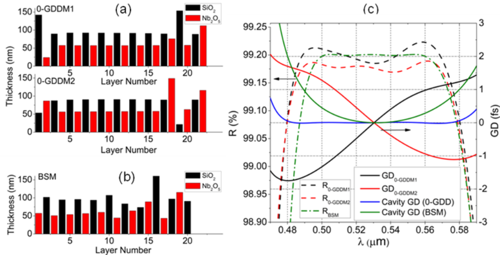
Fig. 2. (a) Structure of a two-mirror zero-GDD mirror set designed for a 40GHz FSR, 100 nm bandwidth (480-580 nm) cavity using Nb 2 O 5 /SiO 2 layer pairs. (b) Structure of a low-dispersion BSM mirror that is individually optimized for the same goal. (c) Calculated reflectivity (dotted curves) and group delay (solid curves) of the zero-GDD mirror pair. The total cavity group delay using the zero-GDD mirror pair (blue) is calculated by taking the dispersion of both mirrors and 7.5 mm of air into account. As a comparison, the total GD (solid) and reflectivity (dashed) of a cavity in vacuum based on two individually-optimized, low-dispersion BSMs is shown in green.
