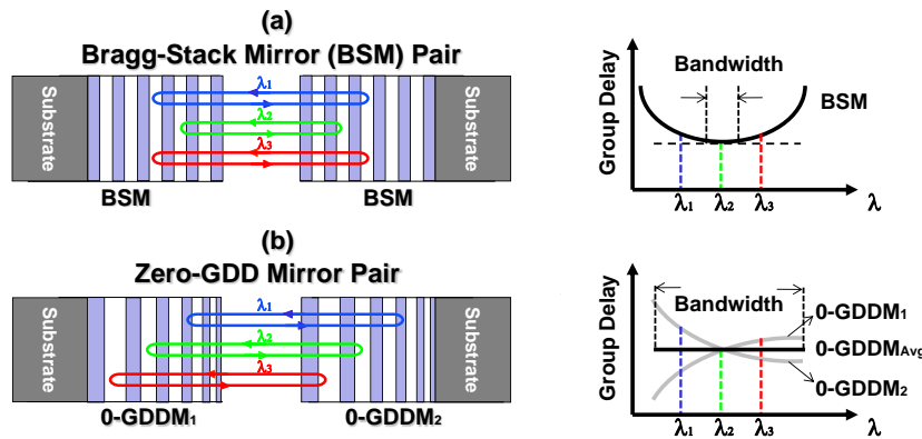
Fig. 1. Schematic of the two-mirror dispersion-free cavity based on (a) Bragg-stack mirror pair and (b) zero-GDD mirror pair. The curves on the right show the individual and average group delay on the cavity mirrors as a function of wavelength.
