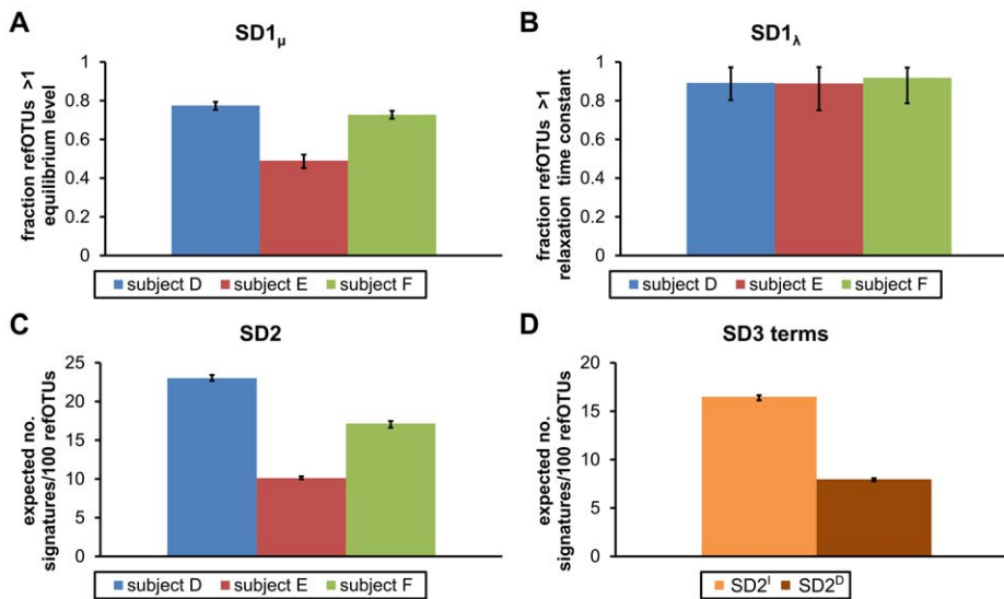
Figure 3. SignatureDiversity scores for gut microbiota of three human subjects treated twice with antibiotics. (A) Intra-signature diversity scores for equilibrium levels ( SD1_{\mu} ), which measure the expected fraction of reference operational taxonomic units (refOTUs) that change equilibrium levels in response to one or more of the antibiotic treatments. (B) Intra-signature diversity scores for relaxation times ( SD1_{\lambda} ), which measure the expected fraction of refOTUs that exhibit different relaxation time constants after the antibiotic treatments. (C) Intra-ecosystem signature diversity scores ( SD2 ), which measure the expected equivalent number of prototype signatures per 100 refOTUs. (D) The inter-ecosystem signature diversity score ( SD3 ), which measures the degree of sharing of prototype signatures across host ecosystems, is a ratio of the SD2^D to the SD2^I score. The SD2^D score is computed on a hypothetical combined ecosystem, in which refOTUs from different subjects probabilistically share prototype signatures. The SD2^I score is a weighted average of SD2 scores computed on each subject separately. doi:10.1371/journal.pcbi.1002624.g003
