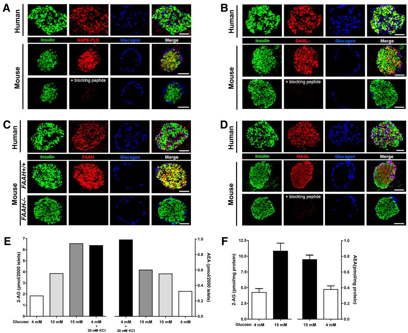
FIG. 2. Identification of intraislet ECS. A and B : Immunostaining for NAPE-PLD ( A ) and DAGL \alpha ( B ) in human and mouse islets. The specificity of anti-NAPE-PLD and anti-DAGL \alpha antibodies was assessed by antigen preabsorption with the corresponding blocking peptides. Scale bar = 50 \mu m. C : Immunostaining for FAAH in pancreatic sections of human and FAAH ^{+/+} and FAAH ^{-/-} mice. Scale bar = 50 \mu m. D : Immunostaining for MAGL in human and mouse islets. The specificity of anti-MAGL antibody was assessed by antigen preabsorption with the corresponding blocking peptides. Scale bar = 50 \mu m. E : Levels of AEA and 2-AG extracted from one lot of human islets exposed to the indicated glucose concentrations with or without KCl for 10 min. The amount of AEA and 2-AG in the samples were determined by calculating the ratio of abundance of AEA or 2-AG to the internal standard abundance. F : Levels of AEA and 2-AG extracted from mouse islets exposed to the indicated glucose concentrations for 10 min. The amount of AEA and 2-AG in the samples were determined by calculating the ratio of abundance of AEA or 2-AG to the internal standard abundance. Data are shown as the mean \pm SEM from two independent experiments. (A high-quality digital representation of this figure is available in the online issue.)
