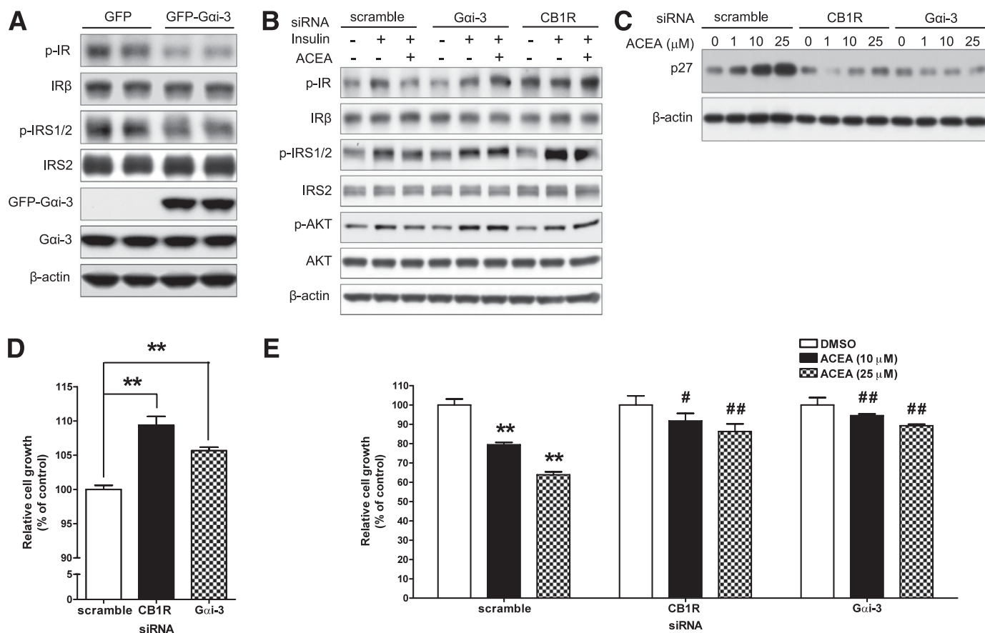
FIG. 8. Inhibitory effects of CB1R on IR signaling require G\alpha_i . A: Effects of G\alpha_{i3} over-expression on p-IR and p-IRS1/2 in \beta -IRWT cells. B: Phosphorylation of IR, IRS1/2, and AKT in \beta -IRWT cells exposed to insulin (10 nmol/L) with ACEA (10 \mu mol/L) or vehicle after transfection of the indicated siRNAs. C: Level of p27 in \beta -IRWT cells exposed to ACEA for 40 h after transfection of the indicated siRNAs. D: Comparison of the proliferation rate between \beta -IRWT cells transfected with scramble, CB1R, or G\alpha_{i3} siRNA. The relative proliferation rate of \beta -IRWT cells was determined 3 days after transfection. Data are shown as the mean \pm SEM from three independent experiments. ** P < 0.01. E: Effects of ACEA on the proliferation of \beta -IRWT cells transfected with the indicated siRNAs. Data are shown as the mean \pm SEM from three independent experiments. ** P < 0.01 vs. vehicle; # P < 0.05; ## P < 0.01 vs. scramble siRNA.
