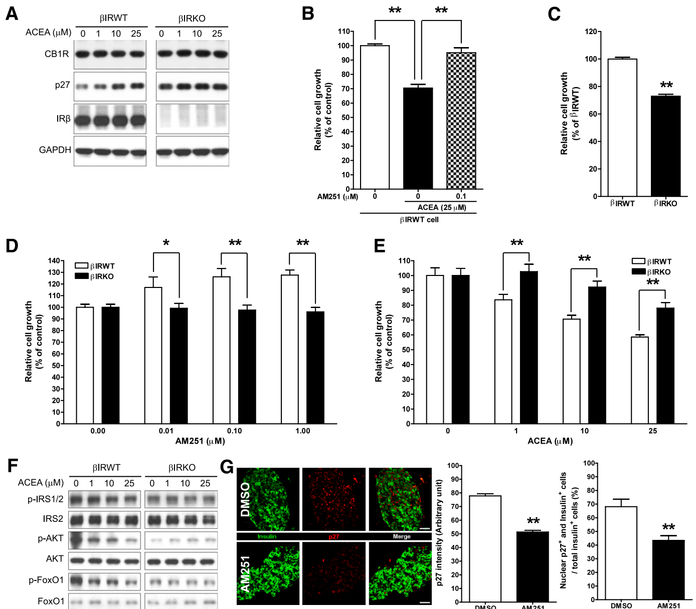
FIG. 5. Inhibitory effects of CB1R on \beta -cell proliferation depends on IR. A: Levels of CB1R, p27, and IR in \beta -IRWT and \beta -IRKO cells exposed to a selective synthetic CB1R agonist ACEA for 40 h. B: Proliferation rates of \beta -IRWT cells exposed to ACEA with or without AM251 for 48 h. Data are shown as the mean \pm SEM from three independent experiments. ** P < 0.01. C: Proliferation rates of \beta -IRWT and \beta -IRKO cells 3 days after plating. Data are shown as the mean \pm SEM from three independent experiments. ** P < 0.01. D: Effects of AM251 on the proliferation of \beta -IRWT and \beta -IRKO cells. Data are shown as the mean \pm SEM from three independent experiments. P < 0.05; ** P < 0.01. E: Effects of ACEA (48 h) on the proliferation of \beta -IRWT and \beta -IRKO cells. Data are shown as the mean \pm SEM from three independent experiments. ** P < 0.01. F: Levels of the indicated proteins in \beta -IRWT and \beta -IRKO cells exposed to ACEA for 40 h. G: Representative immunostaining of insulin and p27 in pancreatic sections from DMSO- and AM251-injected mice. Scale bar = 50 \mu m. Quantification of p27 intensity and nuclear p27 + \beta -cells in islets is shown on the bottom. Data are shown as the mean \pm SEM ( n = 3 per group). ** P < 0.01. (A high-quality digital representation of this figure is available in the online issue.)
