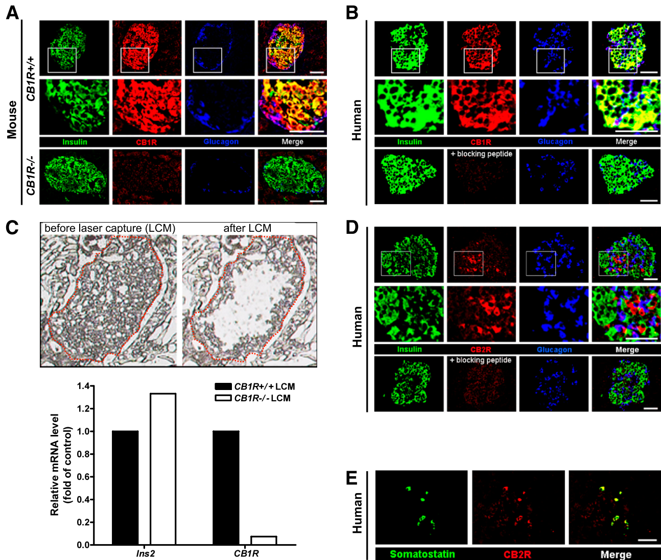
FIG. 1. The presence of CB1R in pancreatic \beta -cells. A: Immunostaining for CB1R in pancreatic sections from CB1R^{+/+} and CB1R^{-/-} mice. Boxed areas are magnified and shown on the bottom panel . Scale bar = 50 \mu m. B: Immunostaining for CB1R in human islets. The specificity of anti-CB1R antibody was assessed by antigen preabsorption with the corresponding blocking peptides. Boxed areas are magnified and shown on the bottom panel . Scale bar = 50 \mu m. C: qRT-PCR amplification of insulin ( ins2 ) and CB1R mRNA from laser-captured \beta -cells of CB1R^{+/+} and CB1R^{-/-} mice. Data were normalized to 18S levels. The upper panel shows a representative image of islets before and after laser capture of \beta -cells. D: Immunostaining for CB2R in human islets. The specificity of anti-CB2R antibody was assessed by antigen preabsorption with the corresponding blocking peptides. Boxed areas are magnified and shown on the bottom panel . Scale bar = 50 \mu m. E: Immunostaining for somatostatin and CB2R in human islets. Scale bar = 50 \mu m. (A high-quality digital representation of this figure is available in the online issue.)
