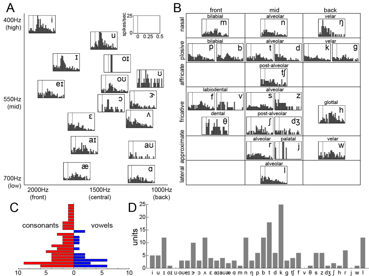
FIGURE IV-4: PSTHS DEMONSTRATE FIRING TO A SUBSET OF PHONEMES.
