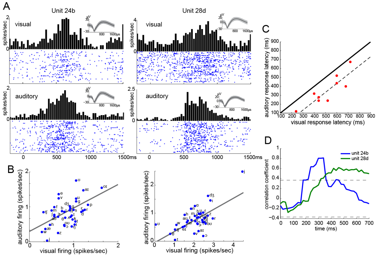
FIGURE IV-8: AUDITORY SINGLE UNITS RESPOND TO WRITTEN WORDS BASED ON PHONEMES IN PRONUNCIATION.
