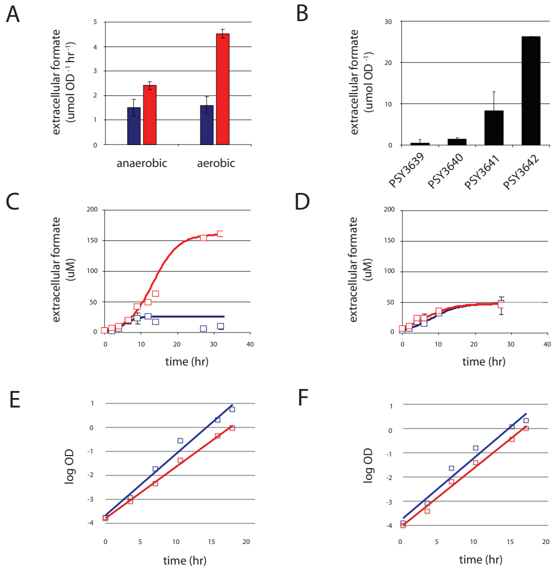
Figure 2.2 Experimental validation of model predictions. Given are formic acid secretion rates under aerobic and anaerobic growth conditions (A), total extracellular formic acid production for several strains (B) including PSY3639 (blue) and PSY3642 (red) grown aerobically (C) and anaerobically (D). Growth rates are given for PSY3639 and PSY3642 grown aerobically (E) and anaerobically (F). Genotypes for strains in B are listed in Table 2.2. Fit-curves in C-F were calculated using logistic regression. Data represent the average of three biological replicates + SD. A paired two-tailed t-test was used to test for statistical significance in (A).
