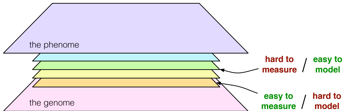
Figure 5.2 Design trade-offs in the meta-ome. Between the genome (the –ome that we can directly manipulate) and the phenome (the –ome that we aim to influence) lie several layers of regulation that impact cell behavior. The distinct properties of each layer affect the biological design cycle. The transcriptome (orange) is easy to measure, but transcript levels are difficult to relate to metabolite concentrations. The metabolome (green) is more difficult to measure, but constraint-based genome scale models can make a priori predictions of the entire metabolic network.
