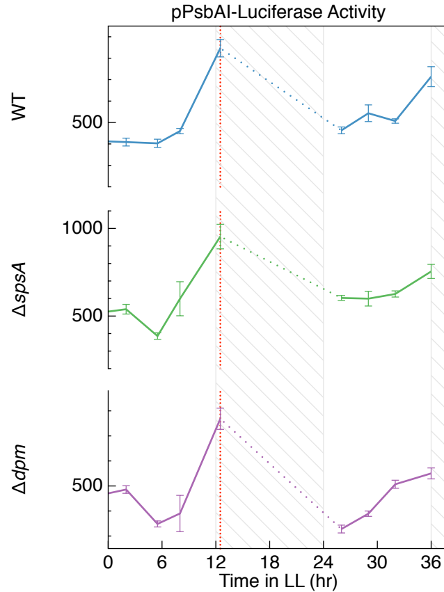
Figure 4.7 pPsbAI -luciferase data corresponding to metabolites measured in Figure 4.4E. Metabolite samples graphed in Figure 4.4E were collected 12.5 hrs into the LL period, as indicated by the dotted red line. No measurements were made during subjective night hours, as indicated by dotted lines. Y-axes are arbitrary luciferase units normalized to the OD at 750 nm. As in Figure 4.4D, the \Delta dpm luciferase signal begins to peak earlier in the subjective day after 24 hours in LL.
