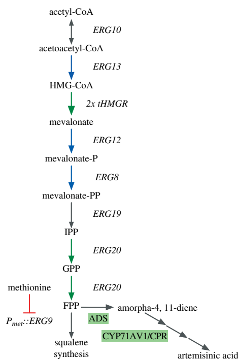
Figure 4. Engineered pathway for artemisinin acid production in S. cerevisiae . Blue arrows indicate enzymes indirectly upregulated by expression of upc2-1 . Green arrows indicate enzymes that were directly upregulated. The red repression arrow indicates that ERG9 was placed under the control of a methionine-repressed promoter, reducing flux to squalene synthesis. Green boxes indicate the exogenous enzymes ADS and CYP71AV1 and the redox partner protein CPR (Ro et al. 2006). CoA, coenzyme A; HMG-CoA, 3-hydroxy-3-methylglutaryl-CoA; IPP, isopentenylpyrophosphate; GPP, geranyl pyrophosphate.
