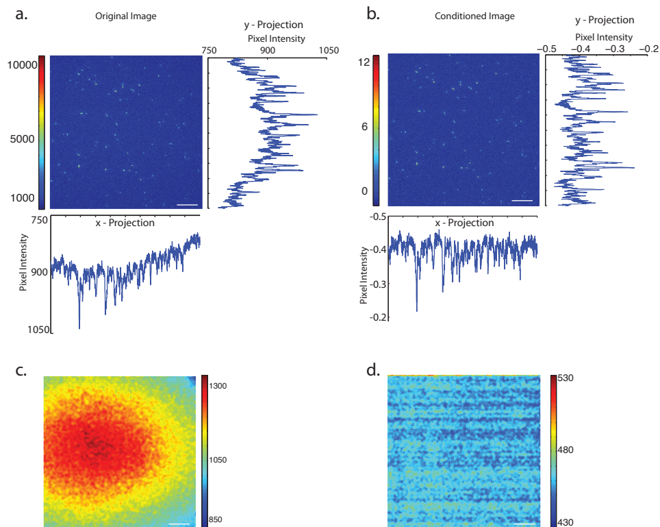
Figure 5.3: The raw image must be conditioned to remove offsets and to correct scaling. For all images, scalebar is 10 \mu\text{m} . (a) The raw red channel image (1000 px by 1000 px) of DNA origami barcodes is shown along with its projections onto the x - and y -axes of the image. The raw image has a large offset and the background varies slowly. (b) The conditioned red channel image is shown with projections onto the x and y axes. The background of the conditioned image has a mean that is constant and nearly zero. (c) Image of only the red channel background, at magnified scale. This image, which has been smoothed by convolution with a Gaussian of width \sigma = 10 px, was taken under the same conditions as a . It contains slide and buffer, without any barcodes. This image is used to correct for uneven illumination, visible as the glowing spot towards the left. (d) Dark red channel image taken with neither slide, nor buffer, nor illumination, is used to correct for DC camera offset. This image has also been smoothed by convolution with a Gaussian of width \sigma = 10 px.
