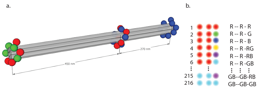
Figure 5.1: Cartoon of DNA origami nanorod barcodes (not to scale). (a) The barcode is composed of a six helix-bundle of DNA, 5 nm in diameter and 720 nm long, decorated at three fluorescing sites with 12 molecules of up to two spectrally distinct fluorophores per site. The barcode has an inherent anisotropy due to the uneven spacing of three fluorescing sites (large gap on the left, smaller gap on the right). The barcode shown is of species RedGreen-RedBlue-Blue. (b) The barcodes use a combination of red (R), green (G), and blue (B) fluorescent molecules, providing a dictionary of six fluorescing symbols at each of the three barcode locations {R, G, B, RG, RB, GB}, for a total of 6^3 = 216 distinct barcode species. In composite images RG appears yellow, RB appears purple and GB appears turquoise.
