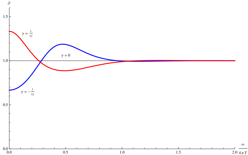
Figure 1: The (dimensionless) conductivity \tilde{\sigma} = g_4^2 \sigma is plotted versus the (dimensionless) frequency \mathbf{\omega} = \omega/(4\pi T) for various values of \gamma (the coupling g_4 is defined in Section 2). Various consistency conditions imply that \gamma \in [-1/12, 1/12] – see discussion surrounding eq. (5.14).
