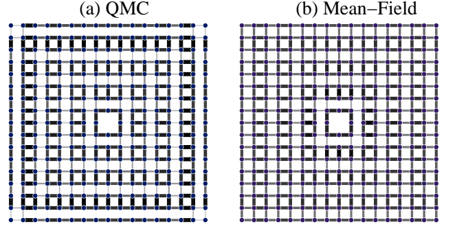
FIG. 2: Comparison of exact quantum Monte Carlo data with saddle-point mean field theory. (a) Dimerization D(x_{ij}) of H_{JQ} with a non-magnetic impurity (a missing spin) on 17 \times 17 system with open boundary conditions. J/Q = 0.1 , T/J = 0.02 . For this value of coupling the system is in the Néel phase. (b) Mean-field results for the generalized charge density \delta\rho_V(r) evaluated on the bonds of a 17 \times 17 open square lattice, evaluated from the saddle point value of V(\mathbf{r}) (which contains an impurity-centered vortex) from \mathcal{S}_V + \mathcal{S}_{\text{imp},V} . We have set a = 0.1 , \tilde{K}_1 = 1 , \tilde{K}_2 = 0 , \tilde{s} = -0.01 , \tilde{u} = 0.3 , \tilde{w} = 0.1 , and the impurity coupling \lambda_1 = 0.5 . The width and darkness of the bonds are related linearly to the plotted quantities. From Fig. 3 it is clear that there is a large contribution from the boundary [23]. Both the effect of the boundary and the single impurity are captured well by the mean field theory. The mean-field theory results are “generic” and the couplings were not picked to tune the agreement with Monte Carlo.
