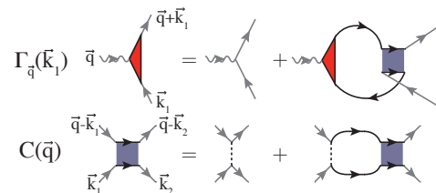
FIG. 3: Diagrams for the vertex function \Gamma and Cooperon C . Solid lines represent bare fermion propagators, dashed lines interactions, and wavy lines external sources. External legs, represented by gray lines, are shown for clarity.
