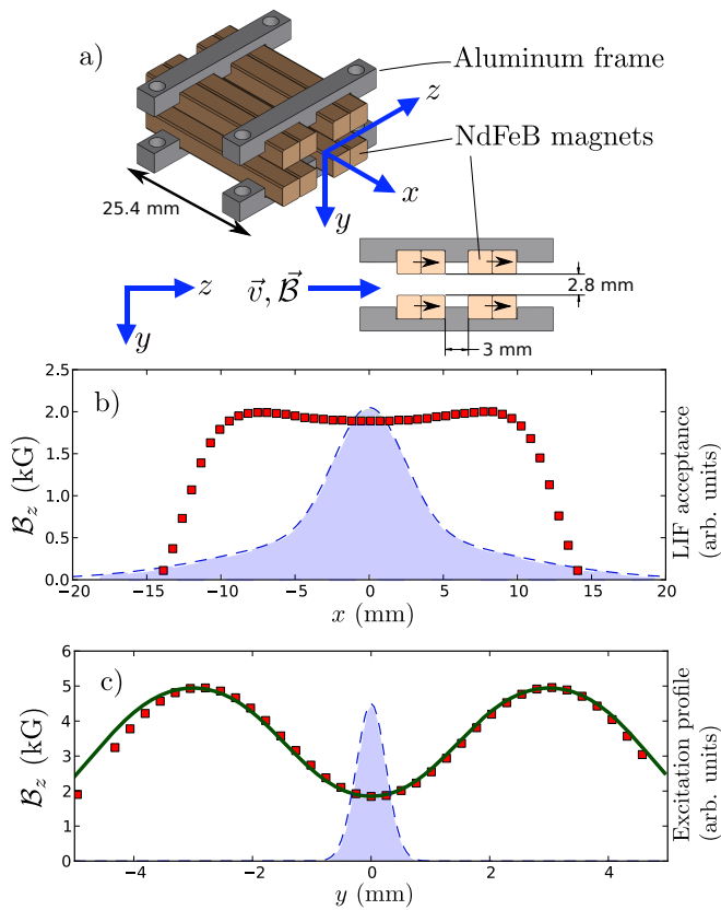
FIG. 1: a) The magnet assembly used in the measurement of \mu_H . Arrows on the NdFeB magnets indicate the direction of magnetization. b) The \hat{z} component of the \mathcal{B} -field, \mathcal{B}_z , measured along the x -axis. The shaded area indicates the calculated acceptance of the LIF detection optics. c) Measured (red squares) and calculated (solid green line) values of \mathcal{B}_z along the y -axis. The shaded area indicates the LIF excitation region, defined by the probe laser's intensity profile.
