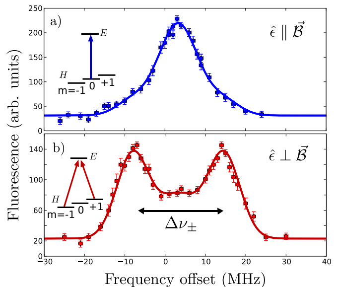
FIG. 2: Spectra of LIF from the H, J = 1 state in a magnetic field \mathcal{B} = 1.9(1) kG, acquired with 16 averages per data point. The x -error bars account for the standard error in the laser's frequency offset (derived from the rms frequency excursion of the lock's error signal) and y -error bars indicate the standard error of the LIF signal due to shot-to-shot fluctuations in the yield of molecules in a pulse. a) The probe laser's polarization \hat{\epsilon} \parallel \vec{\mathcal{B}} ; in this configuration the m_J = 0 sublevel is probed. b) With the laser polarization \hat{\epsilon} \perp \vec{\mathcal{B}} , the m_J = \pm 1 sublevels are probed. The fit to the spectrum in (b) yields \Delta\nu_{\pm} = 22.66(41) MHz for the Zeeman splitting between m_J = \pm 1 .
