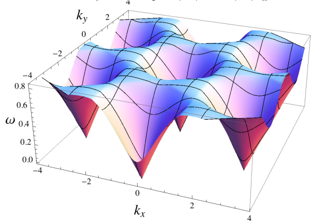
FIG. 7: order: q_1 = -q_2, D/J = 0.03, \kappa = 0.55
