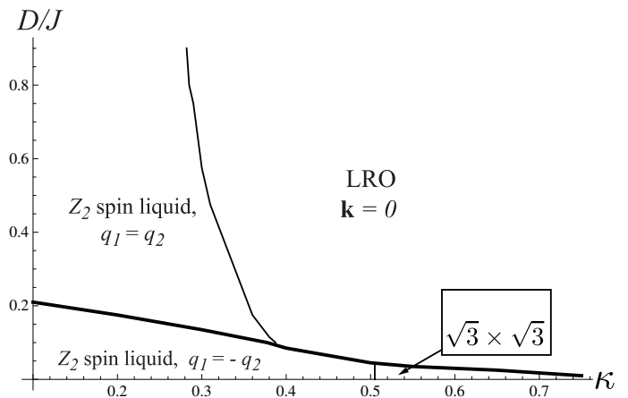
FIG. 3: Phase diagram in the N \rightarrow \infty limit of the \text{Sp}(N) theory. The x-axis shows \kappa = 2S/N and the y-axis D/J . The phases have long-range magnetic order type (LRO), or gapped Z_2 spin liquids. The thick line is a first-order transition, while the thin lines are second-order transitions: the transition to the \mathbf{k} = 0 LRO state is described in Section III. The limit of D/J \rightarrow 0 reduces to the results presented in Ref. 27.
