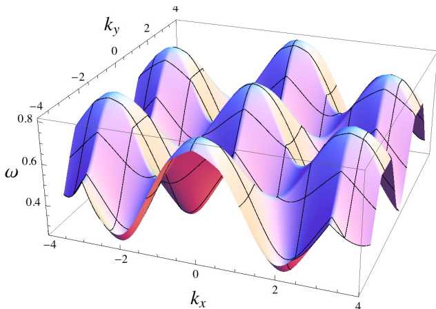
FIG. 6: disorder: q_1 = -q_2, D/J = 0.05, \kappa = 0.3
