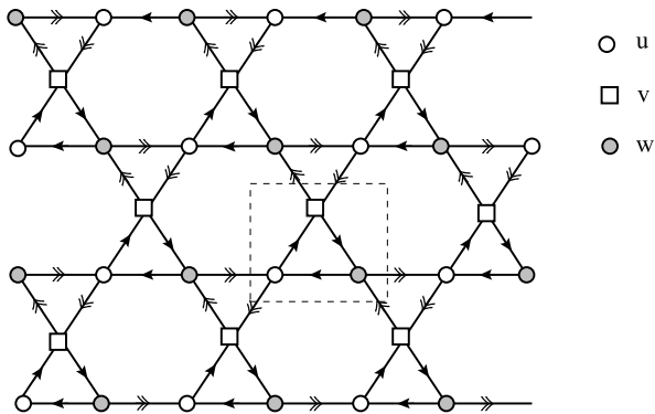
FIG. 2: We take a unit cell of three sites, labeled u , v , w . The arrows indicate the values of the oriented variables q_{ij} . The links with single arrows have q_{ij} = q_1 , while those with double arrows have q_{ij} = q_2 . The P_{ij} are unoriented, and take values p_1 and p_2 on these links respectively.
