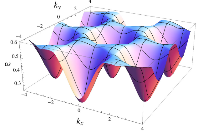
FIG. 4: Momentum dependence of the energy \omega(k) of the lowest excited spinon state of the kagome-lattice quantum antiferromagnet for the q_1 = q_2 state at D/J = 0.3, \kappa = 0.2 . The minimum excitation energy is at \mathbf{k} = 0 and has a finite energy gap.
