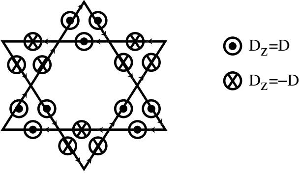
FIG. 1: Staggered DM interaction from triangle to triangle in z -direction as in Ref. 34. The arrowheads indicate D to come out of the plane, whereas the tails denote D to go into the plane. Note that the triangles are summed clock- and anticlockwise, respectively, indicated by the arrows on the bonds.
