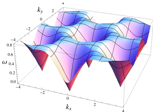
FIG. 5: Dispersion of the lowest excited spinon state for the q_1 = q_2 state at D/J = 0.3, \kappa = 0.4 . The energy gap closes at \mathbf{k} = 0 and condensation occurs.
