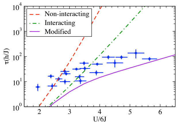
FIG. 14: Doublon decay time as a function of U/6J . The blue circles are the experimental data (cf. Fig. 4). The lines represent theoretical results from resummation with different levels of sophistication from non-interacting Fermions (red dashed line) to the non-crossing approximation with interacting Fermions (green dot-dashed line) to the modified self-energy approximation (purple solid line).
