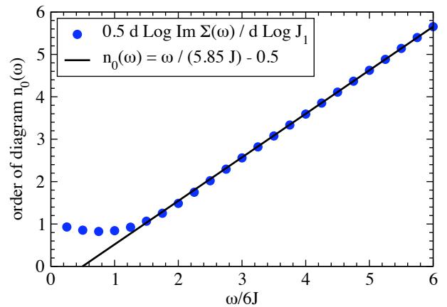
FIG. 11: Order with largest contribution to the Fermion self-energy n_0(\omega) as a function of the frequency \omega . The solid line represents the best linear fit for the high frequency data.
