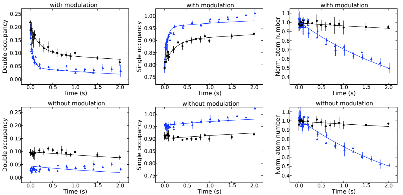
FIG. 2: Time evolution of double occupancy, single occupancy and total atom number for different ratios U/6J . In the upper row, the system was previously excited via lattice modulation. The bottom row shows the reference measurement for the determination of the residual dynamics. The round data points were recorded using a m_F = (-9/2, -7/2) spin mixture with U/h = 1.4 kHz and J/h = 70 Hz, whereas the triangular data points show a (-9/2, -5/2) mixture with U/h = 3.2 kHz and J/h = 100 Hz. The solid lines are simultaneous fits of the integrated population equations of Eq. 4. The total atom numbers are scaled to the initial values. Single occupancy and double occupancy are the fraction of atoms residing on sites of the respective type. Due to different detection efficiencies for hyperfine states the sum of double and single occupancy can be higher than one. Error bars denote the statistical error of at least four identical measurements.
