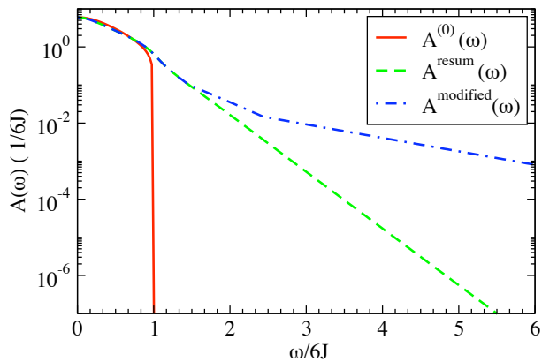
FIG. 12: Fermion spectral functions in different approximations: the free Fermion spectral function ( A^{(0)}(\omega) ); the projected Fermion spectral function obtained as the result of the resummation procedure ( A(\omega) ); the projected Fermion spectral function including corrections for missing diagrams in the resummation procedure (corrected A(\omega) ). The linear slope at high energies on a semi-logarithmic scale shows the exponential transfer of spectral weight due to projection induced interactions.
