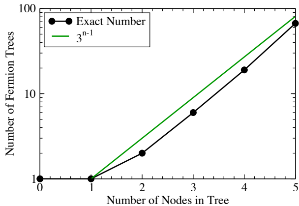
FIG. 18: Dependence of the number of distinct tree diagrams on the number of nodes in the tree.
