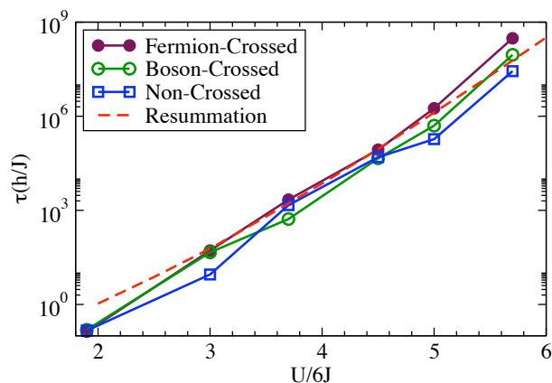
FIG. 16: Comparison of the resummation method and various Golden Rule approximations for calculating the dependence of the Doublon decay time on the interaction strength U/6J (with non-interacting Fermions).
