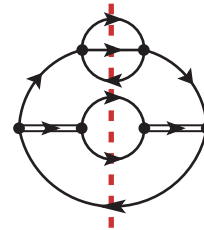
FIG. 5: A Typical doublon self-energy diagram. The double lines are bare doublon propagators while the single lines are bare Fermion propagators. The dashed line cuts the diagram in half and shows the final products of the process represented by this diagram
