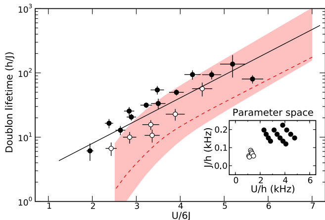
FIG. 4: Semilogarithmic plot of doublon lifetime \tau_D vs. U/6J . The lifetime is extracted from datasets as shown in Fig. 2. Solid and hollow circles denote the (-9/2, -5/2) and (-9/2, -7/2) spin mixture respectively, while the dashed line shows the theoretical result at half filling. The solid line is a fit of Eq. 5 to the experimental data, yielding \alpha = 0.82 \pm 0.08 , whereas for the theory curve the asymptotic slope at large U/6J is \alpha_T = 0.80 . The shaded corridor was obtained by varying the filling factor in the calculation by 0.3. This has only a weak effect on the slope. The inset shows the parameters used to realize the different values of U/6J . Error bars denote the confidence intervals of the lifetime fits and the statistical errors in U/6J . The systematic errors in U/6J and \tau_D = h/J are estimated to be 30% and 25%, respectively.
