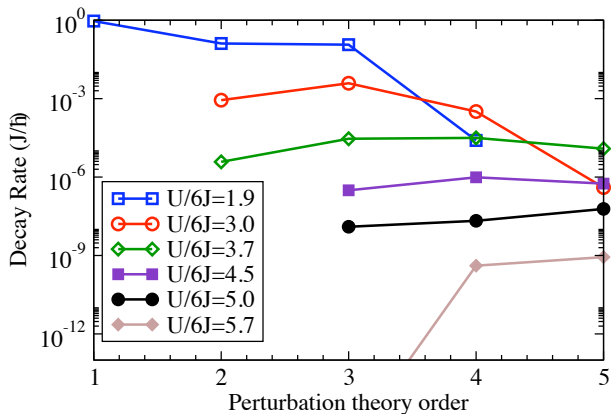
FIG. 15: Decay rate as a function of the order of the perturbation theory computed using Fermi Golden rule. Largest decay rate corresponds to most important order.
