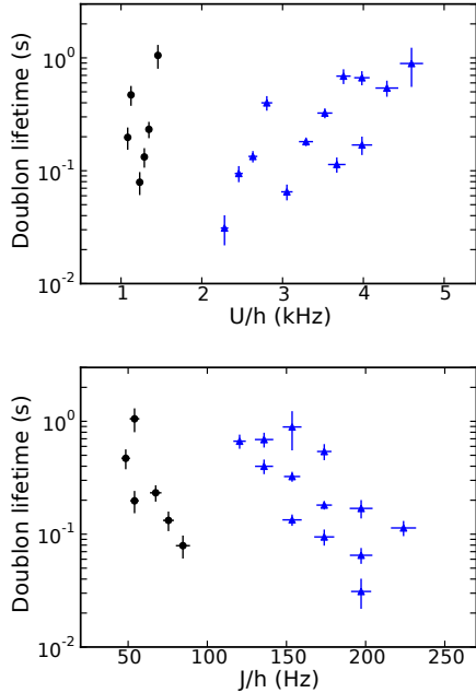
FIG. 3: Doublon lifetime as a function of U and J . The round data points show the fit results to datasets as shown in Fig. 2, obtained with a (-9/2, -7/2) spin mixture while the triangular points correspond to the (-9/2, -5/2) mixture. Error bars denote the confidence intervals of the lifetime fits and the statistical errors in U and J .
