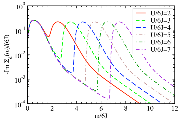
FIG. 13: Doublon self-energy (in the modified Fermion self-energy approximation) for various values of U/6J .
