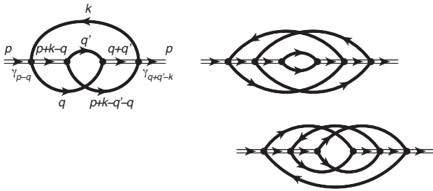
FIG. 7: Typical diagrams for the doublon Green function that are not accounted for in the resummation procedure as they contain crossing Fermion lines. Here, double-lines stand for bare doublon propagators and thick single-lines the full (resummed) Fermion propagator. For reasons explained in the main text, these crossing diagrams do not contribute to the doublon decay, as the vertex factors are not paired and thus average to zero upon momentum integration. To see this, the momenta and a pair of vertices in the first, pretzel-like, diagram are labeled. Notice that the \gamma vertex factors have different momentum labels, these would have been identical for the case of a non-crossed diagram.
