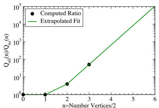
FIG. 19: Correction ratio as a function of the order of the diagram.
