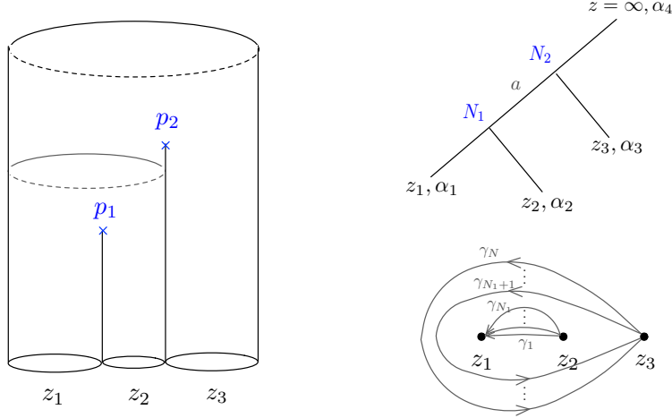
Figure 7: On the left is a light-cone diagram corresponding to the potential (7.5). Together with the eigenvalue distribution N_1 , N_2 = N - N_1 , it maps to the s -channel conformal block shown on the right, with the internal momenta given by a = \alpha_1 + \alpha_2 + N_1 b .
