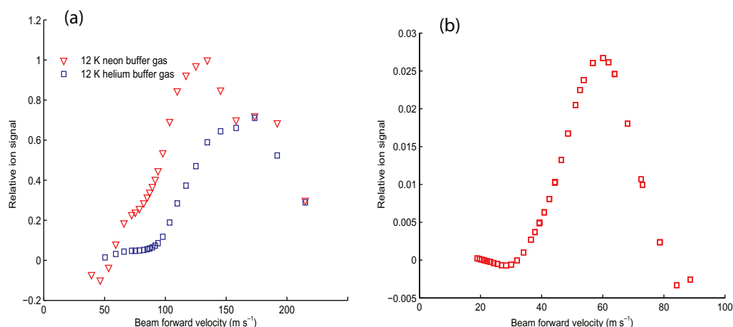
Figure 6. (a) Measured forward velocity distribution of a guided \text{ND}_3 beam using 12 K helium (blue square) and 12 K neon (red triangle) as a buffer gas. The beam using neon contains substantially more low-velocity molecules. Molecules moving faster than \approx 150 \text{ m s}^{-1} are unlikely to be guided by this bent electrostatic guide (bend radius r = 70 \text{ cm} ), although the exact fraction guided depends on the transverse energy of the molecules. The red data (neon) represents a guided beam of about 2 \times 10^{10} \text{ ND}_3 \text{ molecules s}^{-1} at a mean energy of \approx 20 \text{ K} . A background count rate has been subtracted. (b) Velocity distribution at the output of a 70 cm long electrostatic guide with a bend radius of 8 cm. The output of this guide is completely separated from the neon buffer gas, and represents a pure, state-selected, low energy beam. This data represents 3 \times 10^8 \text{ ND}_3 \text{ molecules s}^{-1} , with a mean energy of about 4 K.
