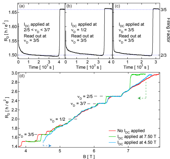
FIG. 3: (a-c) R_D as a function of time measured in the 1 \mu\text{m} constriction at \nu_D = 3/5 after I_{DC} = 10 \text{ nA} was applied at (a) 2/5 < \nu_D < 3/7 , (b) \nu = 1/2 , and (c) \nu_D = 3/5 . (d) R_D as a function of B in the 1 \mu\text{m} constriction. Red trace indicates R_D before I_{DC} has been applied. Green trace indicates R_D after I_{DC} = 20 \text{ nA} has been applied at B = 7.50 \text{ T} . Blue trace indicates R_D after I_{DC} = 34 \text{ nA} has been applied at B = 4.50 \text{ T} .
