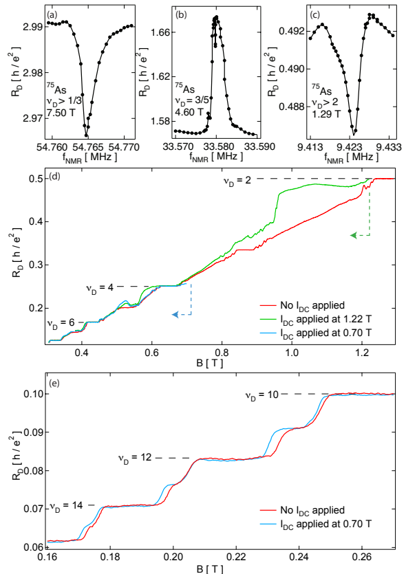
FIG. 4: (a-c) R_D as a function of f_{NMR} in the 1 \mu\text{m} constriction at B = 7.50 \text{ T} , 4.60 \text{ T} , and 1.29 \text{ T} . [24] (d,e) R_D as a function of B in the 1 \mu\text{m} constriction. Red trace indicates R_D before I_{DC} has been applied. Green trace indicates R_D after I_{DC} = 54 \text{ nA} has been applied at B = 1.22 \text{ T} . Blue trace indicates R_D after I_{DC} = 95 \text{ nA} has been applied at B = 0.70 \text{ T} .
