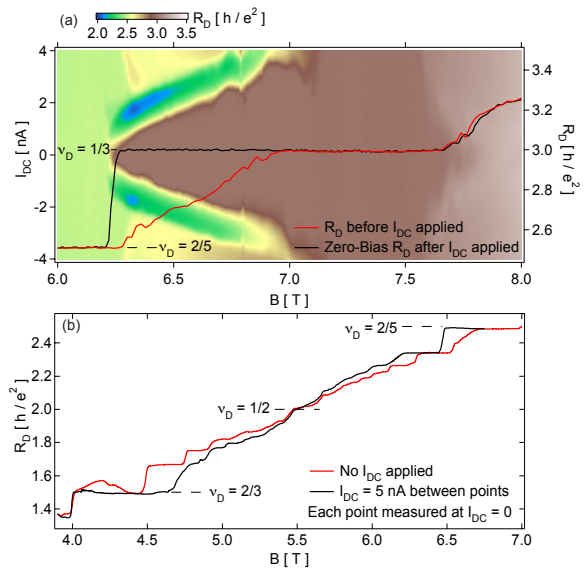
FIG. 2: (a) Diagonal resistance of the QPC, R_{\text{D}} , (Colorscale) as a function of B and I_{\text{DC}} (left scale) in the 750 nm constriction. Traces (right scale) show R_{\text{D}} at I_{\text{DC}} = 0 as a function of B before (red) and after (black) application of I_{\text{DC}} . Black trace is the zero-bias cut through the color plot. (b) R_{\text{D}} as a function of B in the 1 \mu\text{m} constriction before (red) and after (black) application of I_{\text{DC}} = 5 \text{ nA} .
