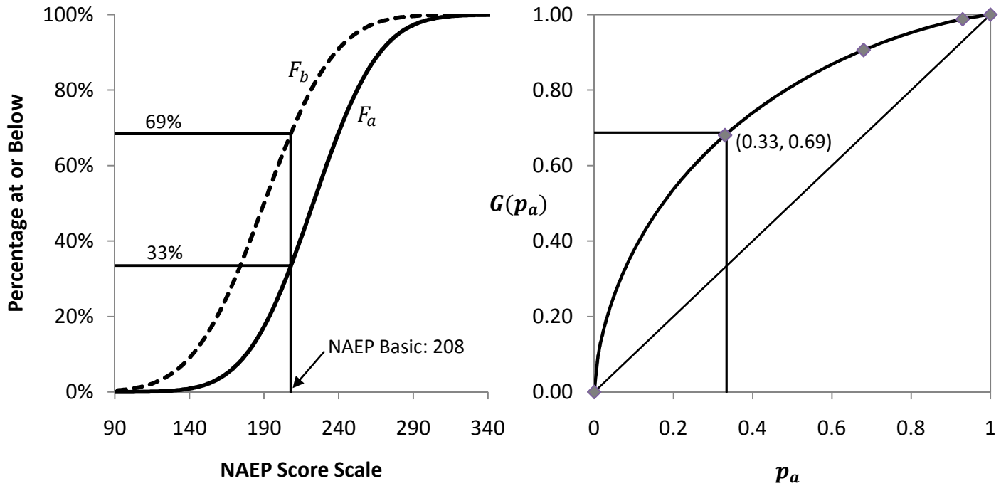
Figure 1. Illustrating the construction of a Probability-Probability (PP) plot from the paired cumulative proportions of distributions. The left-hand panel shows test score distributions for Groups a and b on a common score scale from the National Assessment of Educational Progress (NAEP). The NAEP Basic cut score is also shown, and the percentages at or below that cut score are labeled. The right-hand panel shows the PP plot that represents the paired cumulative proportions from the two distributions at left. The corresponding PP point from the NAEP Basic cut score is identified along with the PP points for the Proficient and Advanced cut scores.
