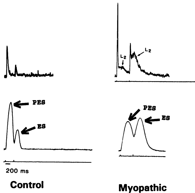
Figure 8. Upper panels demonstrate calcium transients as detected with aequorin. Lower panels demonstrate associated contractile force in isometrically contracting trabeculae carneaee. Using paired electrical stimulation in the case of control myocardium, there is an associated decrease in the amplitude of both the calcium transient and force for the extrasystole (ES). The post-extrasystole (PES) is associated with greater contractile force and a larger calcium transient. In myopathic myocardium, a greater amplitude of the force of contraction was observed for the extrasystole (ES). The amplitude of the first fast component of the [Ca^{2+}]_i signal is greatly diminished compared to the PES. There is a large increase in the amplitude of the second slower calcium transient component ( L_2 ).
