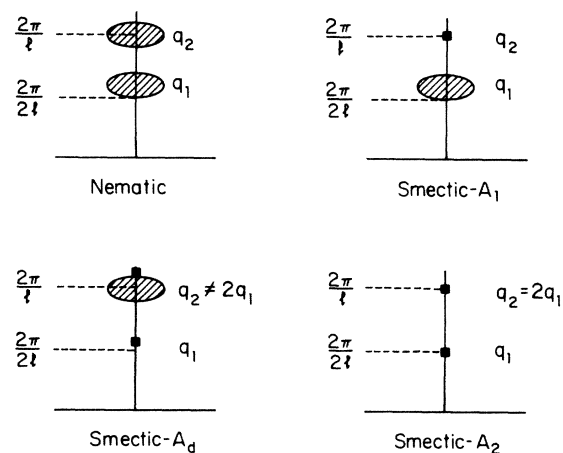
FIG. 2. Diffraction patterns of the polar nematic and smectic- A phases. The vertical axis indicates the q_z direction and the horizontal axis indicates the q_x q_y plane. The small solid squares denote Bragg-like spots and the large ellipses denote diffuse spots. The monolayer ordering ( d = l ) produces the scattering at q_2 and the dipolar ordering ( l < d \leq 2l ) produces the scattering at q_1 .
