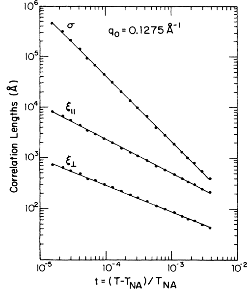
FIG. 13. Power-law fits \sigma = \sigma_0 t^{-\gamma} , \xi_{\parallel} = \xi_{\parallel}^0 t^{-\nu_{\parallel}} , and \xi_{\perp} = \xi_{\perp}^0 t^{-\nu_{\perp}} for the N-A_d transition in DB_6 with c=0.05 and T_{NA_d} as a free parameter. The units for the susceptibility are arbitrary.
