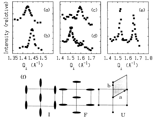
FIG. 2. Scans illustrating diffraction results for the I [(a) Q_z = 0.78 \text{\AA}^{-1} , (b) Q_z = 0 ], F [(c) Q_z = 0.50 \text{\AA}^{-1} , (d) Q_z = 0.24 \text{\AA}^{-1} ], and U [(e) Q_z = 0 ] phases. (f) Schematic illustration of the 2D distorted hexagonal (e.g., rectangular) lattice corresponding to the diffraction results illustrated in (a)–(e). The primitive unit-cell area A_x is indicated by the shaded parallelogram. The peak positions and lattice structure for these three data sets are listed in Table I.
