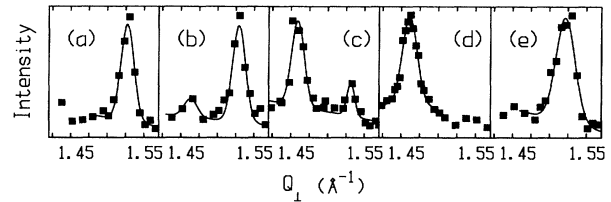
FIG. 3. Illustration of the reversibility of the transition between the U and I phases in regions 3 and 4; Q_\perp scans at Q_z = 0.06 \text{ \AA}^{-1} ; (a) U phase, (b), (c) coexisting U and I phase on compression, (d) pure I phase, and (e) reentrant U phase following expansion. The values of \pi for panels (a)–(e) are 5.90, 6.12, 6.15, 6.33, and 6.06 dyn/cm, respectively.
