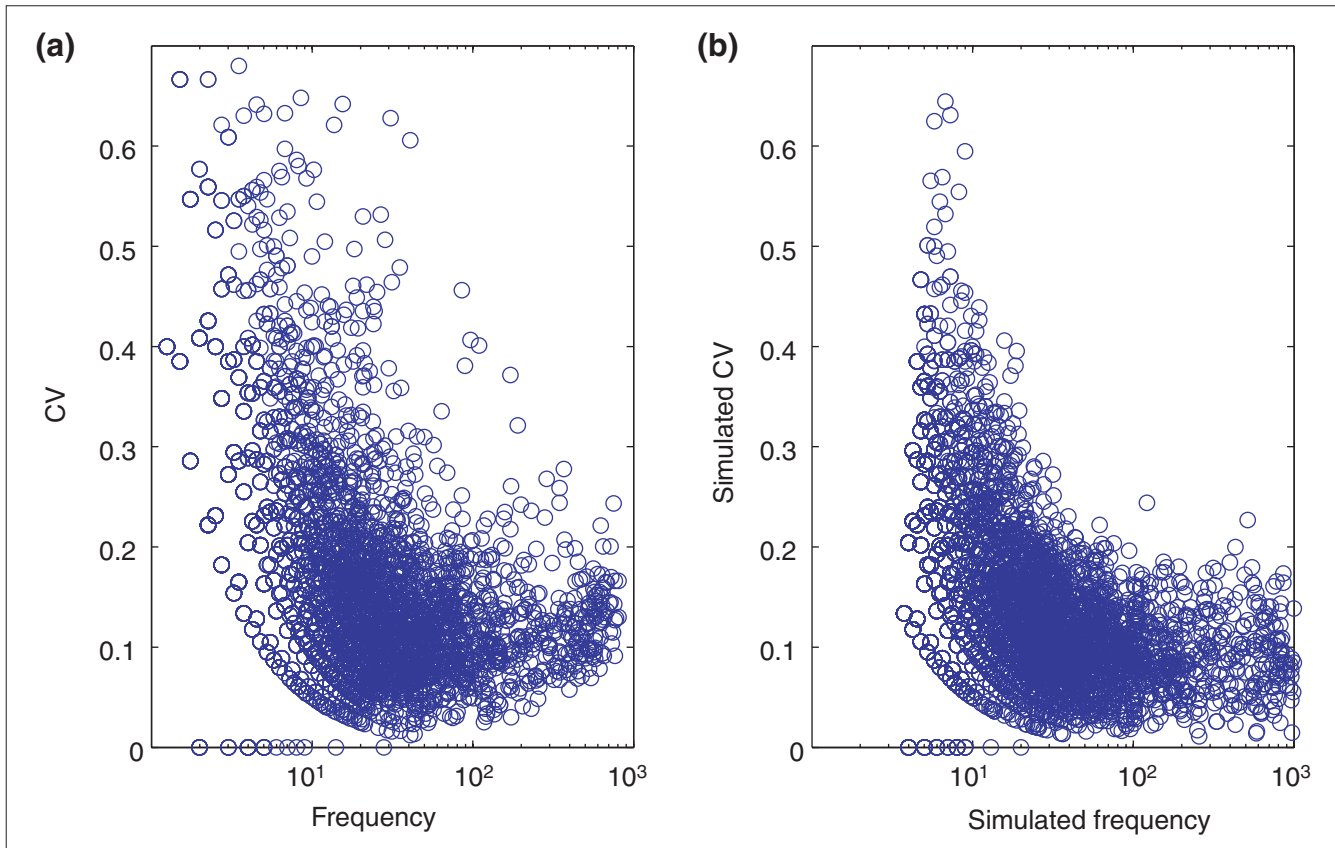
Figure 4 Noise distributions (CV) for the experimental and simulated data sets. (a) 0-hour dataset; (b) simulated dataset. Simulation noise parameters were iteratively estimated from the real data (see Materials and methods). The resulting distributions were sufficiently similar to allow the use of simulations to explore the effects of different sorts of noise on normalization methods.
