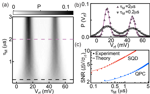
FIG. 3: (Color online) (a) Probability density P of single-shot outcomes, V_{\text{rf}} , (0.7 mV binning) as a function of integration time, \tau_M , of the rf - charge signal v_{\text{rf}} [14]. Measured with SQD, Device 2. The left [right] peak corresponds to the (0,2) [(1,1)] charge state and therefore singlet [triplet] measurement outcomes [5]. (b) Cuts of V_{\text{rf}} along the dashed lines in (a), along with theoretical curves [5]. (c) Signal to noise ratio (SNR), defined as peak separation \Delta V divided by peak width \sigma as a function of measurement integration time \tau_M for QPC1 (Device 1, -89 dBm rf power) and SQD (Device 2, -99 dBm rf power), along with theory curves (see text).
