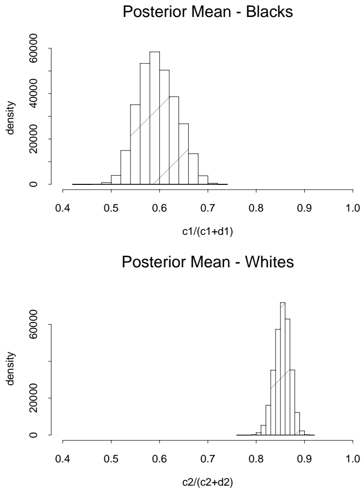
Figure 2: Posterior Distribution of c_b/(c_b + d_b) and c_w/(c_w + d_w) NOTE: The mean of a beta ( a, b ) distribution is a/(a + b) . These figures present the posterior distribution of the second-stage means for blacks and for whites.
