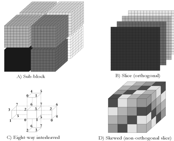
Fig. 3. Common memory organization schemes.
