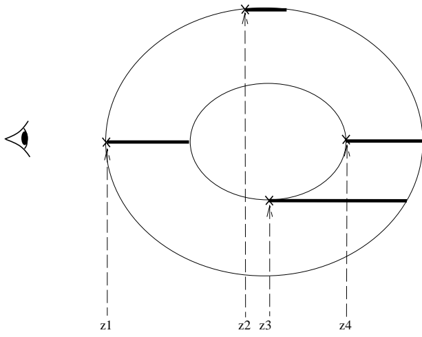
Figure 25. Minimum and maximum segment start depth values for a simple torus shaped volume are at: z[1, 2] for the first segment of all rays, and z[3, 4] for the second segment. Therefore, z[1, 2, 3, 4] define depth planes used to control the order of polygon rasterization. The pseudo planes z = 0 and z = \infty are added to this list.
