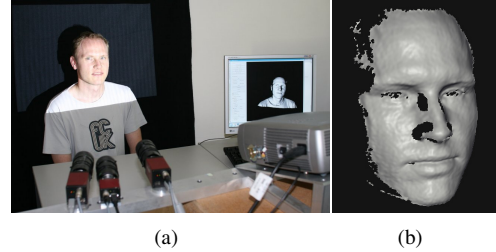
Figure 3. a) Scanning setup. b) Range image after noise and outlier removal.
