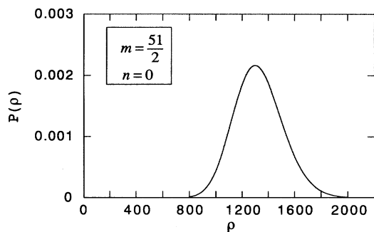
FIG. 1. Plot of the radial probability distribution corresponding to the solution in Eq. (21) with m = 51/2 . The horizontal scale is in units of the “Bohr” radius r_0 [see Eq. (6)]. For a wire current of I = 400 \mu\text{A} , a Landé g factor with |g| = \frac{1}{2} (as in the ground states of sodium), and a mass M equal to the sodium atomic mass, the Bohr radius r_0 = 7.4 \text{ \AA} . This distance is inversely proportional to M and gI . The corresponding binding energy for a spin \frac{1}{2} particle in the state shown is E_B = 6 \times 10^{-10} \text{ eV} . This energy is directly proportional to the mass M and the square of gI (note that the approximate binding energy for a spin 1 particle with m = 25 is about 4 times as large [see Eq. (22)]). It is seen from the figure that the wave function will have a negligible overlap with a wire of diameter 0.5 \mu\text{m} corresponding to a radius r = 340r_0 .
