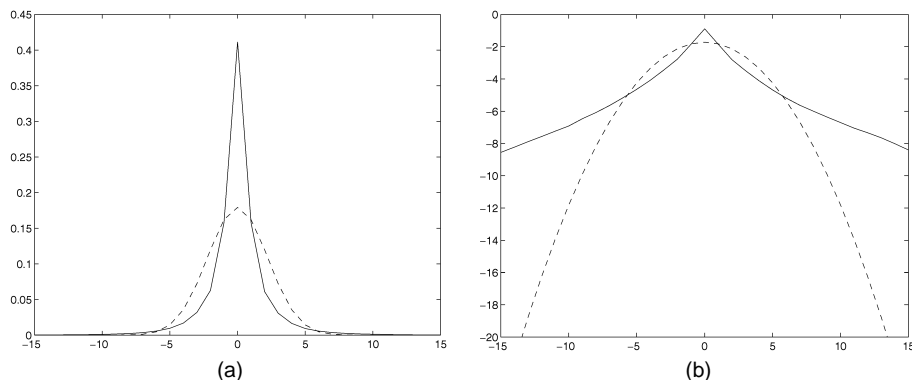
Fig. 5. (a) The histogram of |\nabla_x I| plotted against Gaussian curve (dashed) of same mean and variance in domain [-15, 15] . (b) The logarithm of the two curves in (a).
