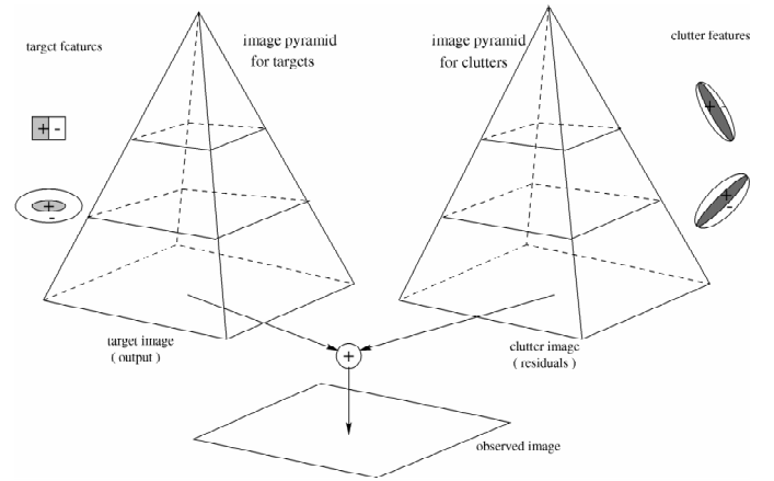
Fig. 15. The computational scheme for removing noise and clutter.
