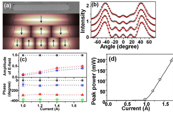
FIG. 4 (color online). (a) SEM image of the facet of a QCL with a 22- \mu\text{m} -wide active region, and simulations showing from top to bottom the electric field of \text{TM}_{00} , \text{TM}_{02} , and \text{TM}_{04} modes of the device; the arrows in the figure indicate the polarization of the field. (b) Measured far-field intensity distributions of the device (open circles) and their fits (solid lines) at driving currents of 1.7, 1.4, 1.2, and 1.0 A (from top to bottom). The curves are shifted vertically for clarity. (c) Electric-field amplitude (upper panel) and phase (lower panel) of the transverse modes used to fit the far-field data in (b). Open circles: \text{TM}_{00} mode; open triangles: \text{TM}_{02} mode; open squares: \text{TM}_{04} mode; open diamonds: \phi_{\text{TM}_{00}} + \phi_{\text{TM}_{02}} - 2\phi_{\text{TM}_{04}} . Dotted lines are used to guide the eyes. Error bars indicate the range of individual parameter changes that will lead to a root mean square deviation of 0.05 between the experimental data and the fits. (d) Light output versus current curve for the device. The dots indicate the operating conditions at which the different near- and far-field measurements were performed.
