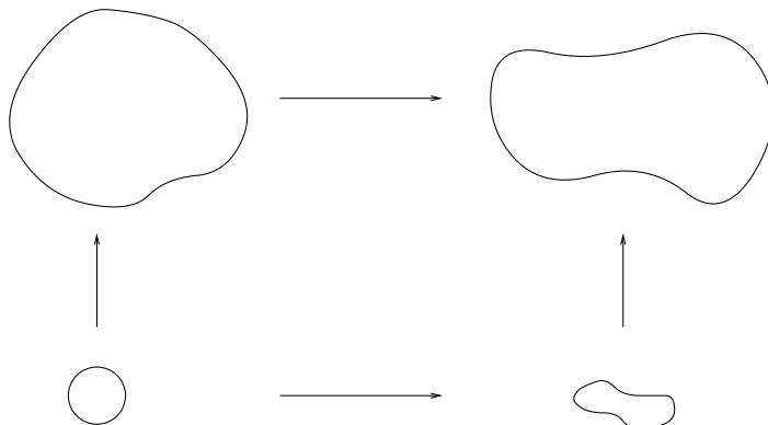
Figure 3. Proof of quasiconformality of \psi .
