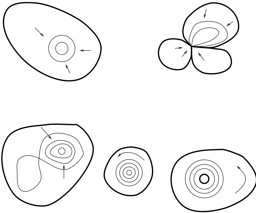
Figure 1. The five types of stable regions.
