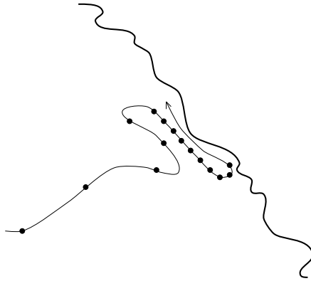
Figure 2. Orbit tending to the Julia set.
