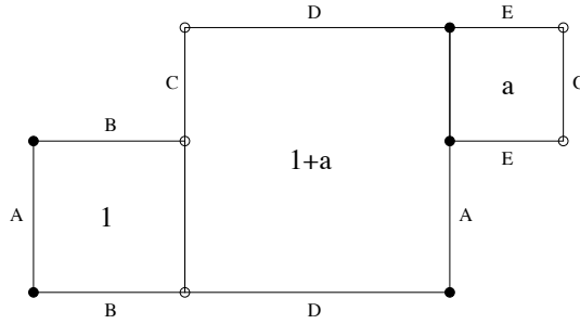
Figure 6. The polygon S(a) and its gluing pattern.
