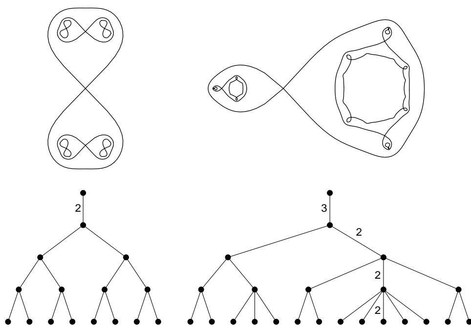
Figure 1. Critical level sets of G(z) for f(z) = z^2 + 2 and f(z) = z^3 + 2.3z^2 , and the corresponding combinatorial trees. The edges mapping with degree > 1 are indicated. The Julia set of z^2 + 2 is a Cantor set, while the Julia set of z^3 + 2.3z^2 contains countably many Jordan curves.
