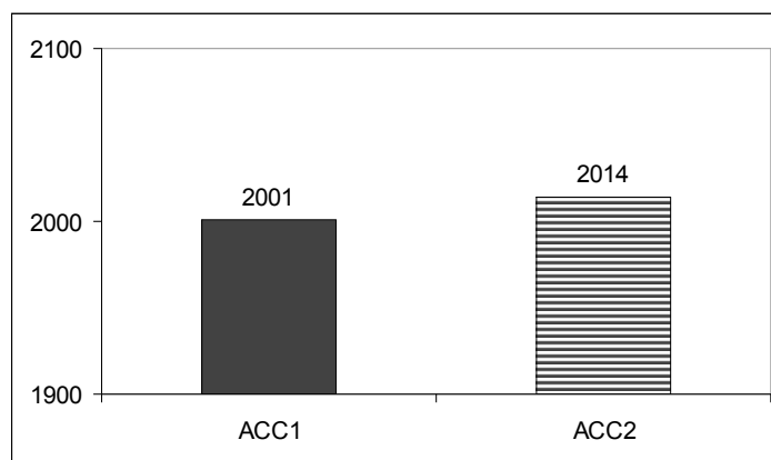
Figure 1 Reading time results, ACC1 and ACC2 (Kwon & Polinsky 2006)
