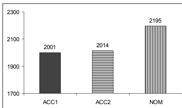
Figure 2 Reading time, collapsed, three control constructions (Kwon & Polinsky 2006)
