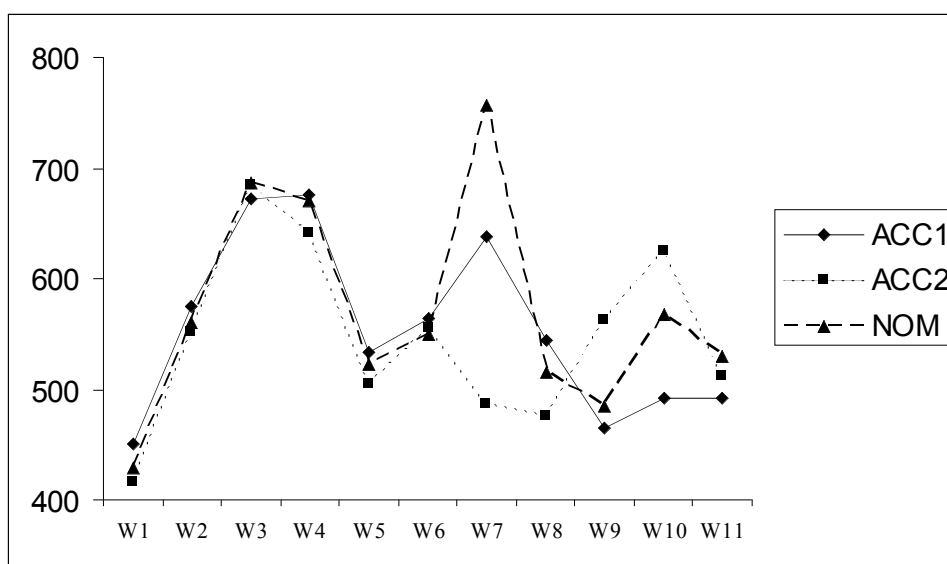
Figure 3 Reading time course, three control constructions
