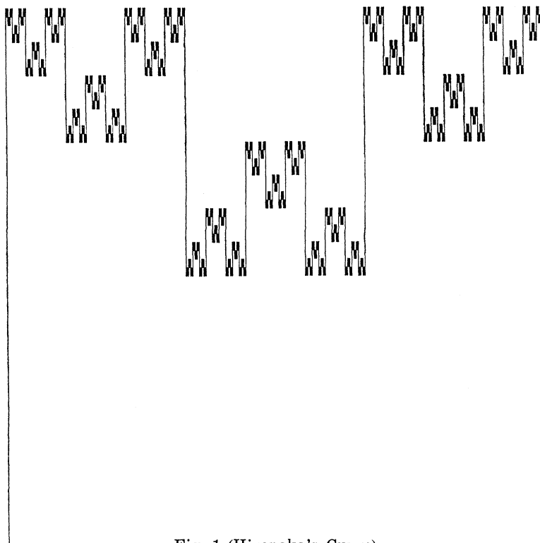
Fig. 1 (Hironaka's Curve)
