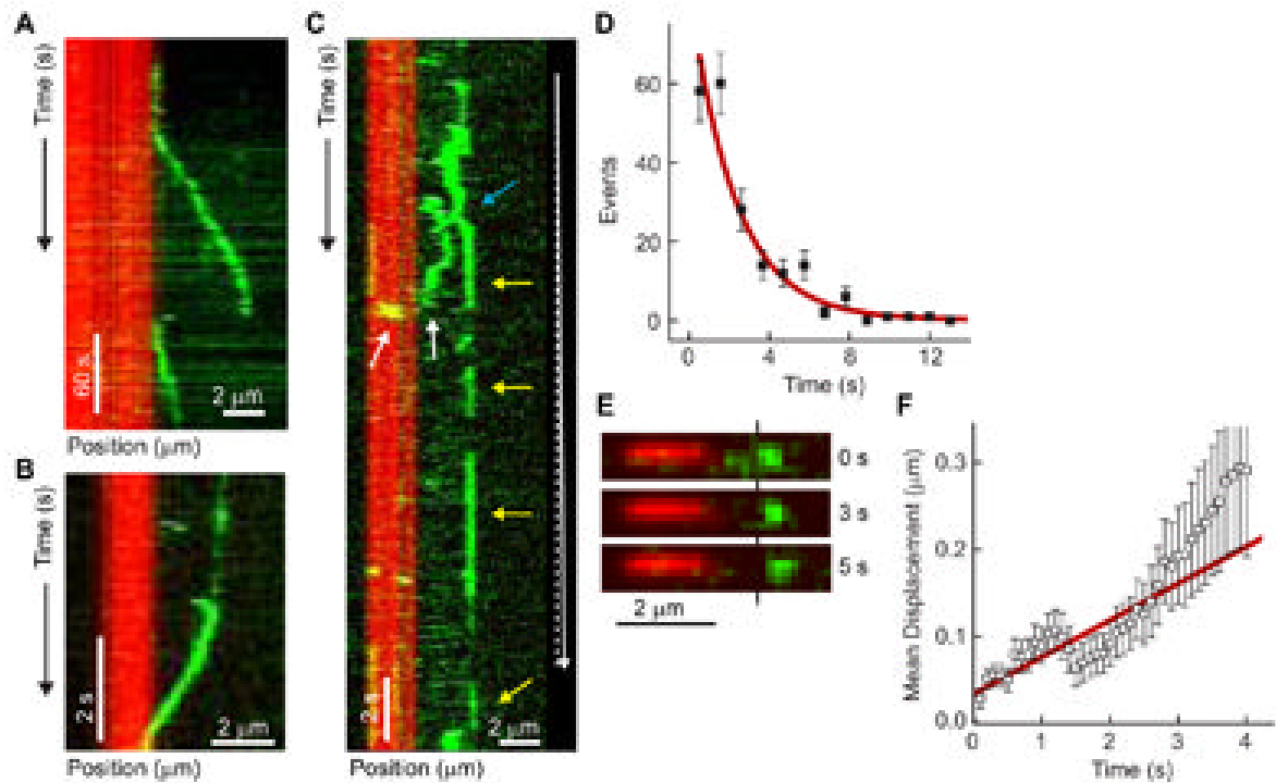
Figure 2. XMAP215 at dynamic microtubule ends
