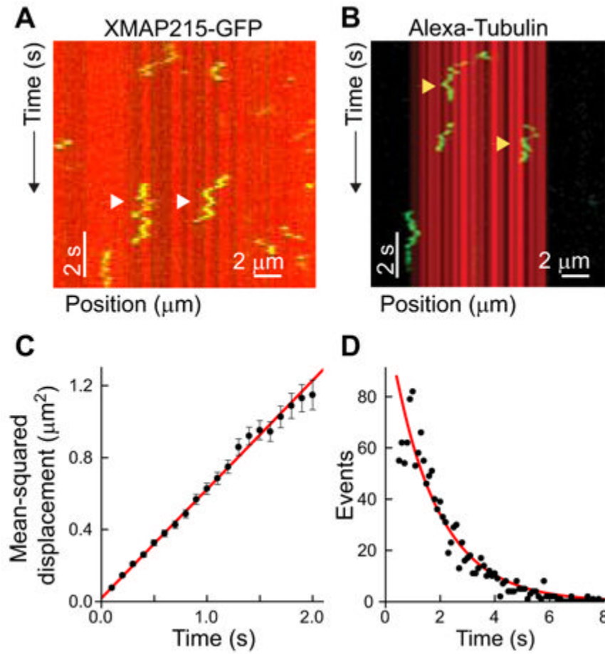
Figure 4. XMAP215 targets one tubulin to the microtubule end by lattice diffusion (A) Kymograph depicting the diffusion of XMAP215-GFP alone on a GMPCPP microtubule (white arrows). (B) Kymograph depicting the XMAP215:tubulin complex diffusing on the microtubule (yellow arrows). Note the similarity to (A). (C) Plot of mean-squared displacement versus time for XMAP215-GFP against the time interval over which it was measured. A linear curve fit to the data yields a diffusion coefficient, D , of 0.3 \pm 0.01 \mu\text{m}^2 \cdot \text{s}^{-1} . Error bars are the SEM of the squared displacement values ( n = 1383 ). (D) Histogram of durations of XMAP215-GFP microtubule interactions. An exponential curve fit, corrected for photobleaching, yields a mean lifetime of the interactions, \langle t \rangle , of 2.45 \pm 0.21 \text{ s} .
