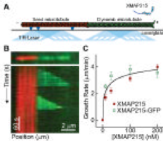
Figure 1. XMAP215 promotes microtubule growth and binds plus ends
