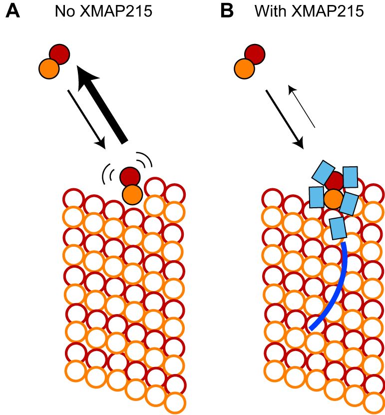
Figure 6. Model diagram for tubulin polymerization by XMAP215
